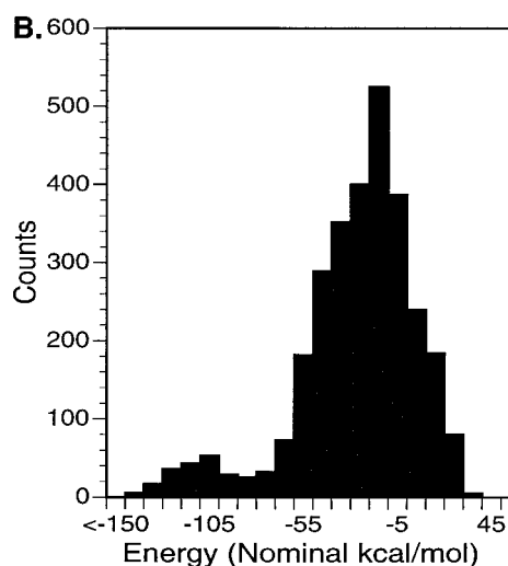
FIGURE 8 Probability distribution function of interpeptide interaction energy for the odd ( A ) and even ( B ) interfaces, averaged over all helices and all time frames.
