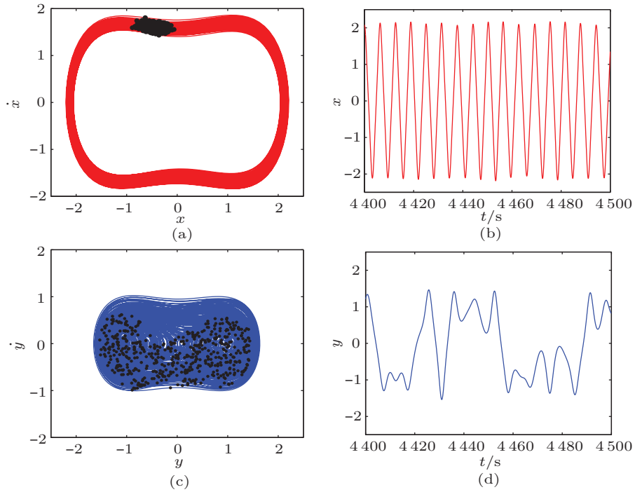
Fig. 6. Phase portraits (lines) with Poincaré points (black points) projected into planes x-\dot{x} in (a) and y-\dot{y} in (c), and time series of x(t) in (b) and y(t) in (d) for \omega = 1 .
