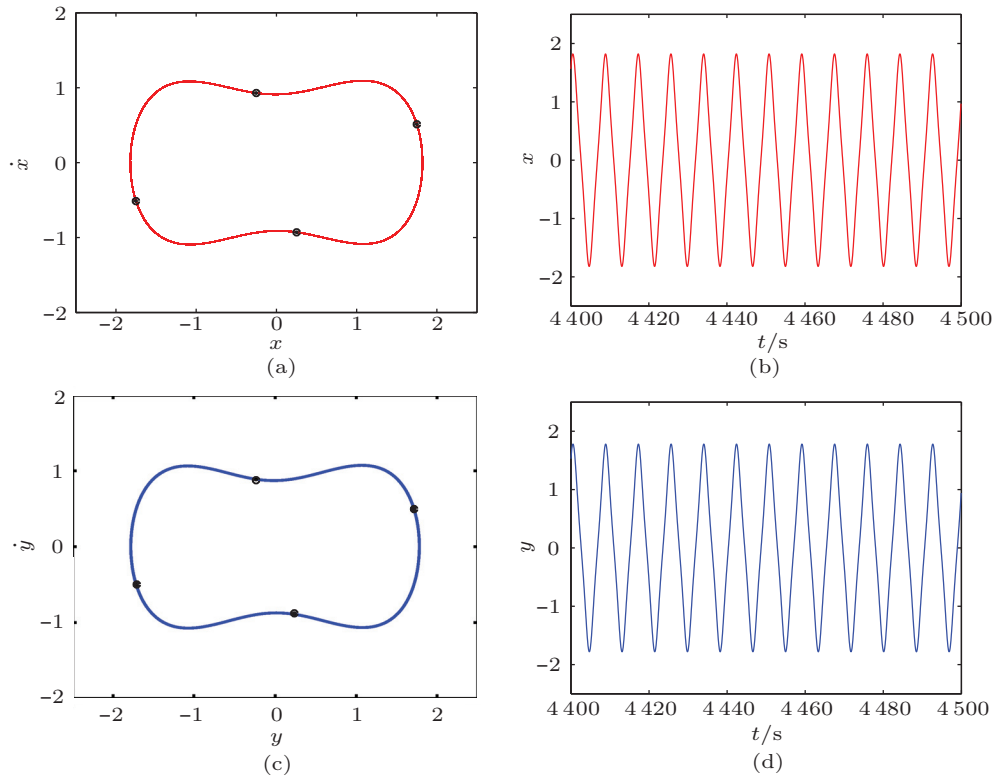
Fig. 5. Phase portraits (lines) with Poincaré points (black points) projected into planes x-\dot{x} in (a) and y-\dot{y} in (c), and time series of x(t) in (b) and y(t) in (d) for \omega = 0.7 .
