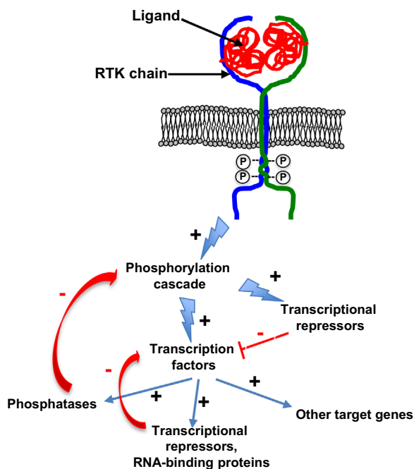
Fig. 3. The negative feedback loops regulating RTK activation. The window of time required for inducing mRNA and protein synthesis after RTK activation is between 15 and 90 min. These mechanisms are tightly regulated by negative feedback loops. Indeed, the phosphorylation cascade induced by RTK activation leads to the activation of numerous transcription factors and simultaneously their repressors. The translocation of the various transcription factors can also induce the expression of transcriptional repressors or phosphatases, which in turn can repress the corresponding transcription factors and/or the upstream kinase activities. +: activation; -: repression.
