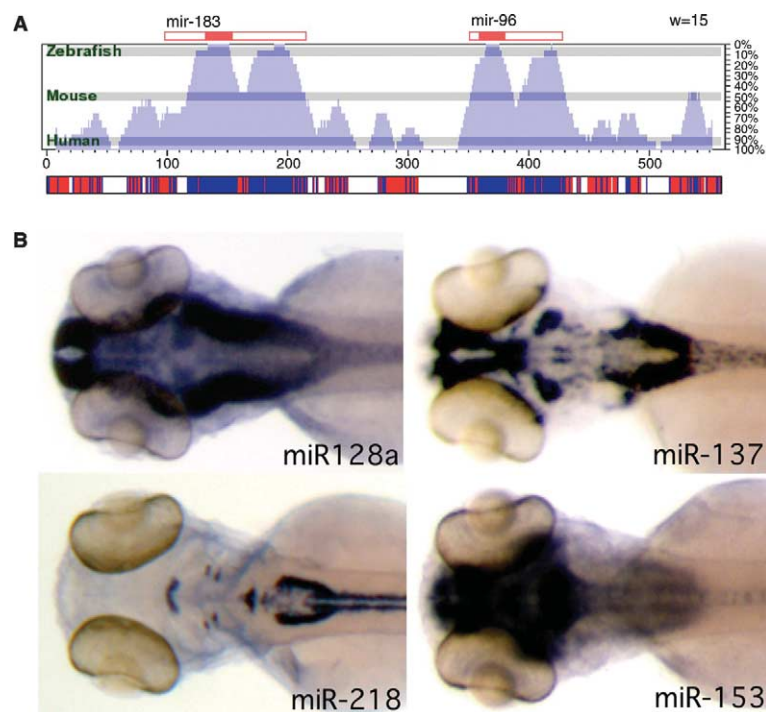
Fig. 2. Vertebrate miRNAs in zebrafish. (A) Phylogenetic conservation of two clustered vertebrate miRNA genes. miRNA regions (indicated by the red boxes) are more conserved than flanking sequences. See [9] for details. (B) Example expression patterns of conserved brain-specific miRNAs in zebrafish embryos. Adapted with permission from [42].
