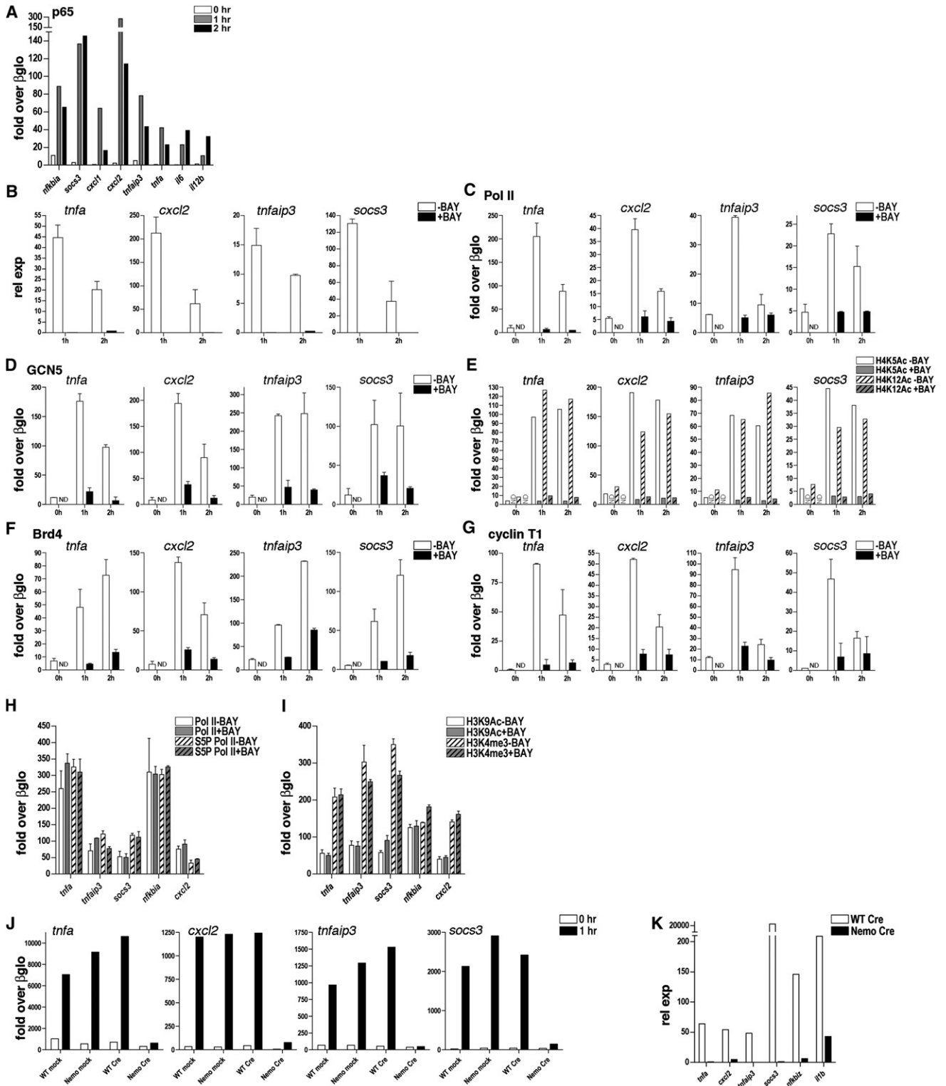
Figure 6. Signal-Dependent NF- \kappa B Activation Is Required for Inducible H4K5/8/12 Acetylation, Brd4 Recruitment, and P-TEFb Recruitment (A) BMM \phi s were stimulated for 1 or 2 hr with LPS and analyzed by ChIP (p65). (B–G) BMM \phi s were left untreated (white bars) or treated with BAY-11087 (black bars), stimulated with LPS for 1 or 2 hr, and analyzed by (B) RT-qPCR or by (C–G) ChIP at the 3' end (total Pol II) or at the TSS (GCN5, H4K5Ac, H4K12Ac, Brd4, cyclin T1). ND indicates not done. (H and I) BMM \phi s were treated with or without BAY-11087 and NF- \kappa B inhibitor II and analyzed by ChIP (total Pol II, S5-P Pol II, H3K9Ac, H3K4me3).
