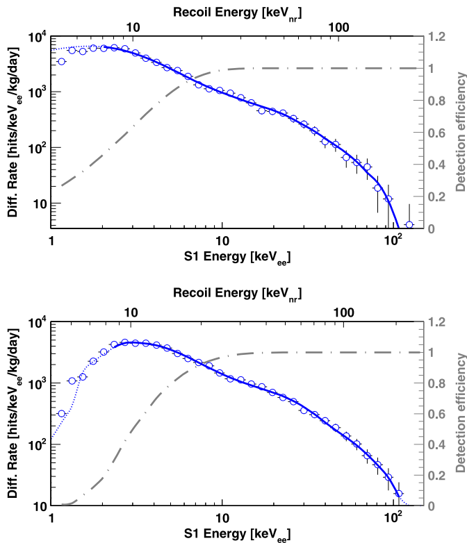
Fig. 2. The differential spectrum of the primary scintillation of single scatter nuclear recoils from the 2008 (top) and 2010 (bottom) Am–Be data. Also shown are the results from a detailed Monte Carlo simulation (solid lines) considering an energy dependence of \mathcal{L}_{\text{eff}} as in Fig. 3 and the corresponding nuclear recoil energy scale. S1 energies below 2.0 keV ee (FSR) and 2.5 keV ee (SSR) are not used to obtain the fit and are shown as extrapolations only (dotted). Superimposed is the detection efficiency (dash-dotted).
