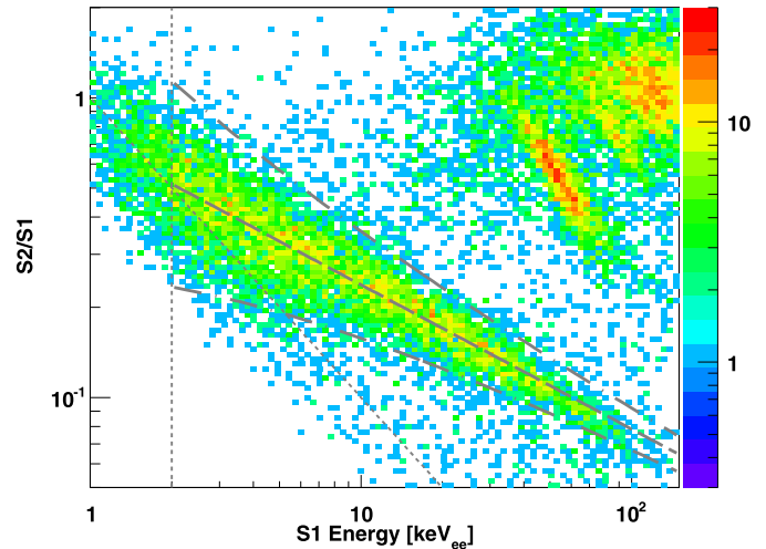
Fig. 1. The discrimination parameter S2/S1 for the nuclear recoil response to an Am–Be neutron source. The colour scale indicates the counts for a 4.9 h exposure in the FSR configuration. The analysis thresholds for scintillation ( S1 ) and ionisation ( S2 ) are indicated by dotted lines. The centroid of the population and the \pm\sigma contour used for this analysis are indicated by the dashed and dash-dotted lines. The 40 and 80 keV ee inelastic populations can also be seen. (For interpretation of the references to colour in this figure legend, the reader is referred to the web version of this Letter.)
