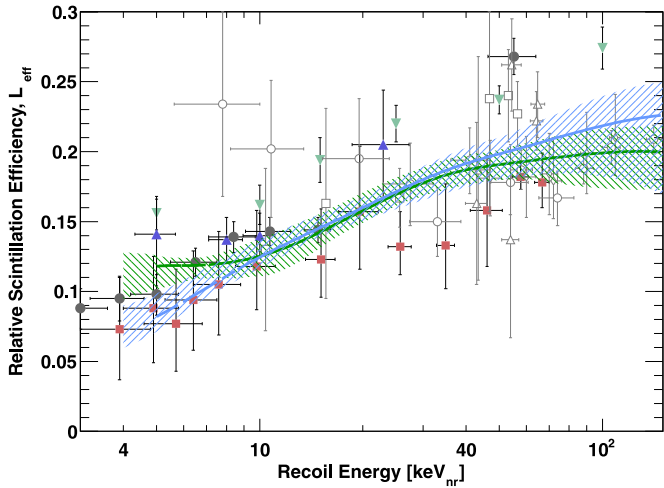
Fig. 3. The energy-dependent relative scintillation yield for nuclear recoils \mathcal{L}_{\text{eff}} (solid lines) for the two ZEPLIN-III datasets, including relevant 68% C.L. bands (FSR: green \llcorner , SSR: blue \llcorner ). Below the analysis range (corresponding to \sim 7 – 9 keV nr ), the scintillation yield is indicated as dashed lines. Also shown are previous published measurements using mono-energetic neutron beams: (●) [10], (■) [11], (▲) [25], (○) [26], (△) [27], (▽) [28] and (◇) [21], or obtained using a similar Monte Carlo matching procedure (▼) [7]. (For interpretation of the references to colour in this figure, the reader is referred to the web version of this Letter.)
