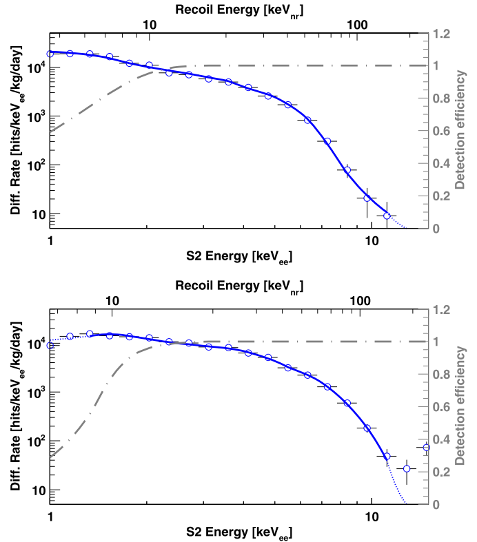
Fig. 4. The differential spectrum of secondary scintillation signals from single scatter nuclear recoils from the two datasets (top: FSR; bottom: SSR). Also shown are the Monte Carlo data (solid lines) considering an energy dependence of \mathcal{Q}_y as in Fig. 5 and the corresponding nuclear recoil energy scale. S2 energies below 1.0 keV ee (FSR) or 1.2 keV ee (SSR) and above 11 keV ee are not used to obtain the fits and are shown only as extrapolations (dotted). Superimposed are the detection efficiencies (dash-dotted) as obtained by the primary scintillation signal S1 (see Fig. 2) and converted into S2 energy using the mean correlation between the two channels.
