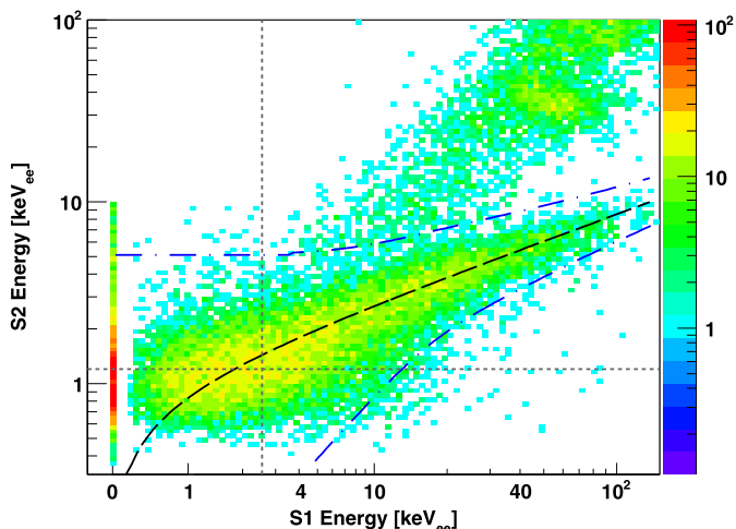
Fig. 6. The nuclear recoil response to Am-Be neutrons in the SSR configuration including events below the previous analysis threshold for S1 and S2 (dotted lines). The colour scale gives the counts for a 5.9 h exposure. Also indicated are the \pm 3\sigma contours to the centroid of the neutron recoil population (dashed and dashed-dotted) and their extension sub-threshold. (For interpretation of the references to colour in this figure legend, the reader is referred to the web version of this Letter.)
