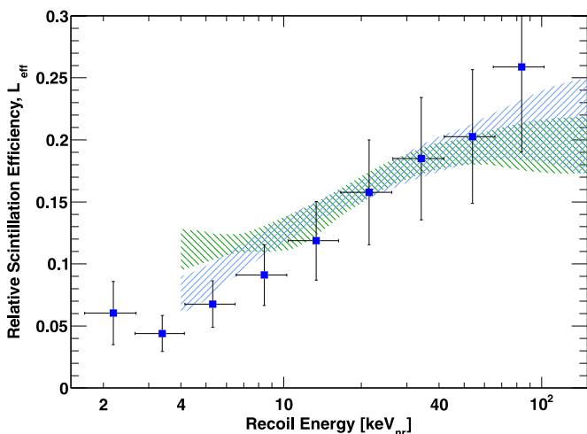
Fig. 7. The relative scintillation yield for nuclear recoils \mathcal{L}_{\text{eff}} as determined by extending the event selection to S2-only events for the SSR Am-Be data. Also shown are the results obtained using the Monte Carlo fitting method, as in Fig. 3.
