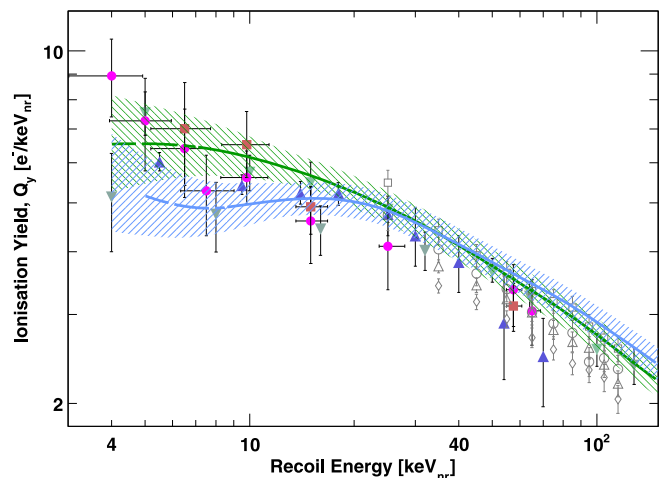
Fig. 5. The ionisation yield \mathcal{Q}_y for nuclear recoils as derived from the FSR (green \llcorner ) and SSR (blue \llcorner ) datasets including relevant 68% C.L. bands. Results below the analysis range are indicated by dashed lines. Also shown are previous measurements at 1.0 kV/cm (●) and 4.0 kV/cm (■) from Ref. [11], at 2 kV/cm (□), (△), 0.3 kV/cm (○) and 0.1 kV/cm (◇) from Ref. [21] and spectra obtained using similar Monte Carlo matching procedures at 0.73 kV/cm (▲) [7] and (▼) [29]. (For interpretation of the references to colour in this figure, the reader is referred to the web version of this Letter.)
