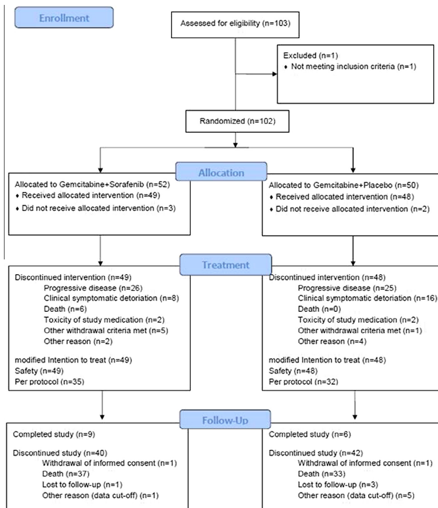
Fig. 1. CONSORT chart.
