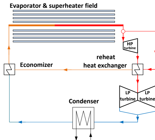
Fig. 3. Indirect reheat configuration
