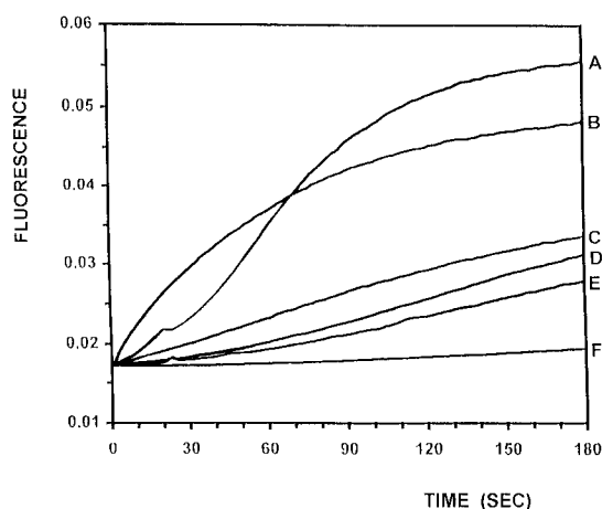
Fig. 6. Time-dependent polymerization of F-actin under the influence of EWAM fragments. (F) Actin control. At low molar ratios to actin E1-3 apparently promotes actin polymerization about 10-fold faster than E(1-295) and 100-fold faster than E(1-185), as the polymerization curves are parallel for the 1:1000 ratio of E1-3 (D), the 1:100 ratio of E(1-295) (C) and the 1:10 ratio of E(1-185) (E). Comparing a 1:100 ratio of E1-3 to actin (A) and a 1:10 ratio of E(1-295) to actin (B) it becomes obvious that E(1-295) overcomes the lag phase of polymerization more efficiently than E1-3.
