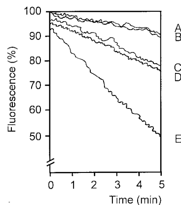
Fig. 5. Severing activity by EWAM and its fragments measured by the dilution-induced depolymerization assay. Fluorescence of F-actin was taken as 100% and that of G-actin as 0. F-actin control (A) and E(1-185) in a molar ratio of 1:5 to actin (B) are similar in the first 5 min after dilution. E(1-295) is shown in a 1:10 ratio to actin (C) and E1-3 as 1:30 (D) and 1:10 (E).
