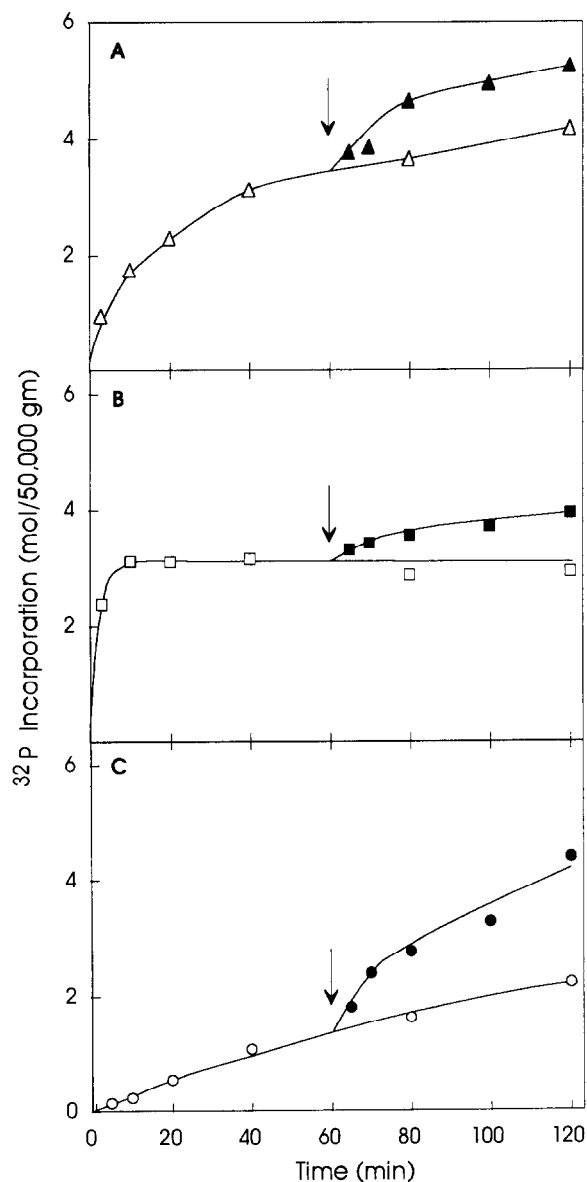
Fig. 3. Phosphorylation of tau by a combination of CK-1, CaM kinase II, Gr kinase, and GSK-3. Tau was separately phosphorylated by CK-1 ( \Delta ,A), CaM kinase II ( \square ,B) and Gr kinase ( \circ ,C). After 60 min ( \downarrow ), aliquots of the reaction mixtures were separately removed and supplemented with GSK-3 ( \blacktriangle , \blacksquare , \bullet ) and the incubations continued.
