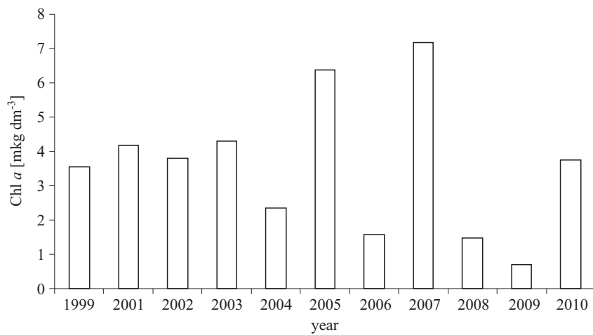
Figure 6. Current changes (1999–2010) in summer chlorophyll a in Petrozavodsk Bay (Lake Onega)
