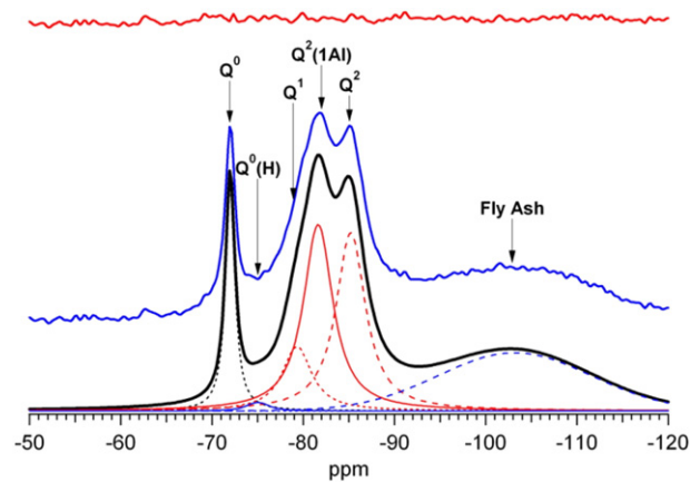
Fig. 12. Single-pulse ^{29}\text{Si} MAS NMR spectrum (middle) for a water-activated 50% wPc-50% pfa blend hydrated for 9 years at 25^\circ\text{C} . The result of the deconvolution of the spectrum is shown at the bottom and the residual at the top. The C-A-S-H peaks have chemical shifts of -79.3 for Q^1 , -81.6 for Q^2(1\text{Al}) , and -85.2 for Q^2(0\text{Al}) ; there is a small Q^{0\text{H}} peak at -75.0 ppm. The spectrum was acquired over 5760 scans using a pulse recycle delay of 5 s, a pulse width of 6 \mu\text{s} and an acquisition time of 20.5 ms.
