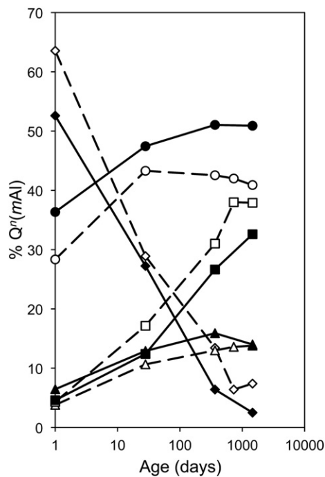
Fig. 14. The % of Si that is present as Q^0 (alite and belite; diamond), Q^1 (circle), Q^2(1Al) (triangle) and Q^2(OAl) (square) in neat white Portland cement pastes plotted against age for activation with water (open symbols) and KOH solution (filled symbols).
