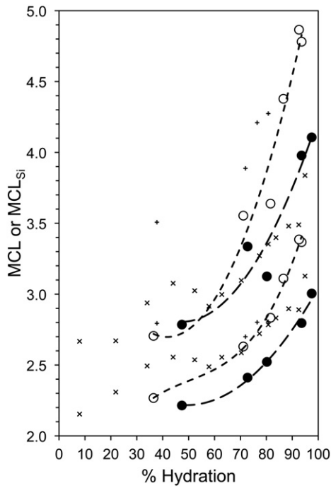
Fig. 16. Variation in MCL and MCL Si with % hydration for neat white Portland cement activated by water (open circles) or KOH solution (filled circles). In both cases, the upper data are MCL and the bottom data are MCL Si . The dashed lines are guides for the eye. For comparison, equivalent data are included for water-activated neat white Portland cement from [47] (x; w/c = 0.5; 20 °C) and from [106] (+; w/c = 0.425; 25 °C).
