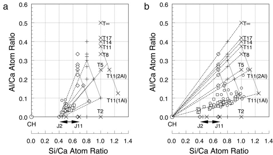
Fig. 21. Al/Ca against Si/Ca atom ratio plots of TEM-EDX analyses of Ip ( \square ) and Op ( \circ ) C-A-S-H present in (a) the water-activated and (b) the KOH-activated neat cement pastes hydrated for 28 days at 25 °C.
