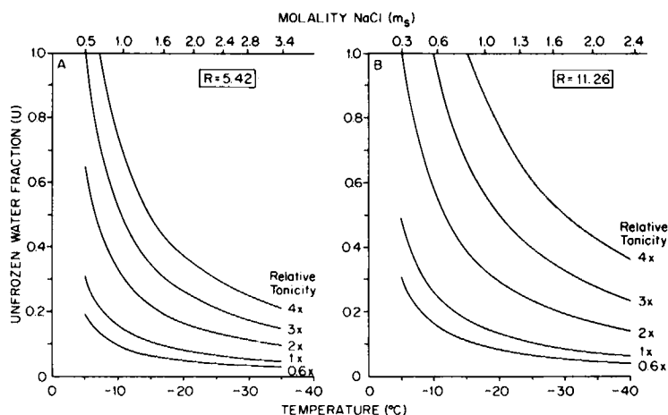
FIGURE 6 U vs. temperature for glycerol-NaCl-water solutions: (A) R = 5.42; (B) R = 11.26. In both A and B the initial concentration of NaCl ranges from 0.6 to 4 times isotonic. The compositions of the solutions before freezing are given in Table I. The upper abscissas show the molality of NaCl ( m s ) that is present in the unfrozen portions of the solution at the indicated temperatures.
