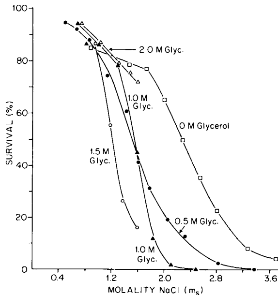
FIGURE 3 Survival (percent unhemolyzed cells) of human erythrocytes as a function of the molality of NaCl ( m_s ) to which they are exposed after being frozen at 1.8^\circ\text{C}/\text{min} to various subzero temperatures while suspended in solutions of the indicated molarity of glycerol in isotonic NaCl.
