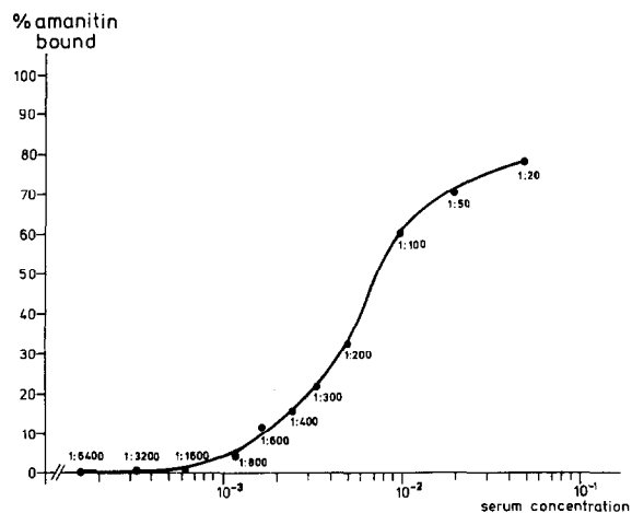
Fig. 1. Titer of amanitin binding proteins in the serum of a rabbit. Final dilution of the serum in the assay plotted versus % of radioactive amanitin bound (100% = 1.7 pmol- 3 H)- O -methyl-demethyl- \gamma -amanitin = 5200 cpm).
