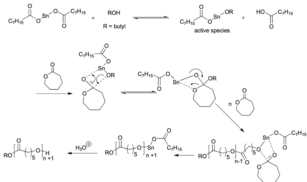
Scheme 2. Most common synthetic routes to PCL.
