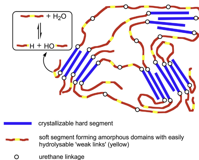
Scheme 7. Multiblock copolymer thermoplastic architecture, with crystallizable poly[(3- R -hydroxybutyrate)- co -(3- R -hydroxyvalerate)] hard segments and poly[( \epsilon -caprolactone)- co -glycolide] soft segments containing easily hydrolysable ester bonds.
