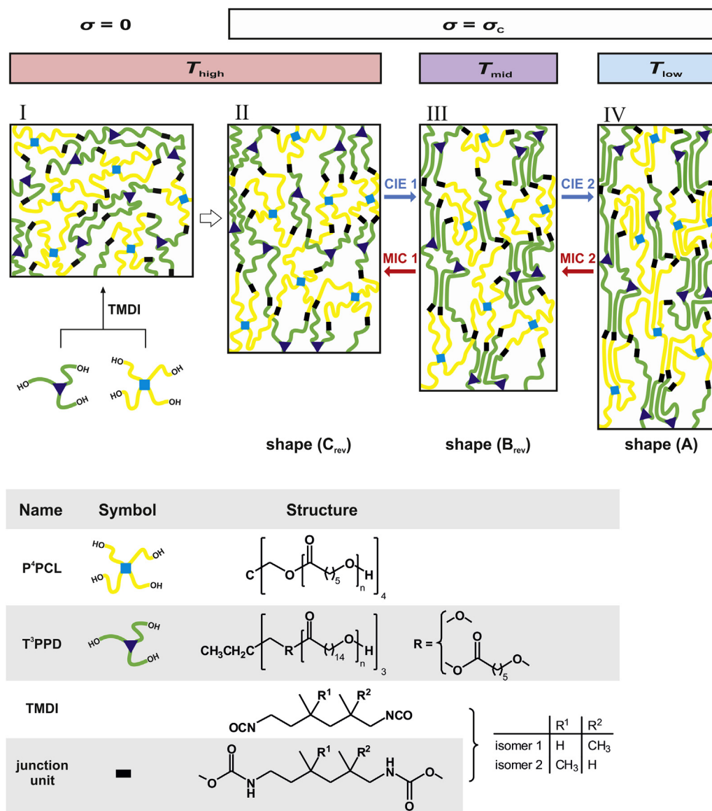
Scheme 8. Reversible shape change phenomena showing contraction or elongation of co-PEU networks prepared from star-shaped PCL and PPD. Taken from Ref. [159]. Copyright © 2010 WILEY-VCH Verlag GmbH & Co. KGaA, Weinheim.
