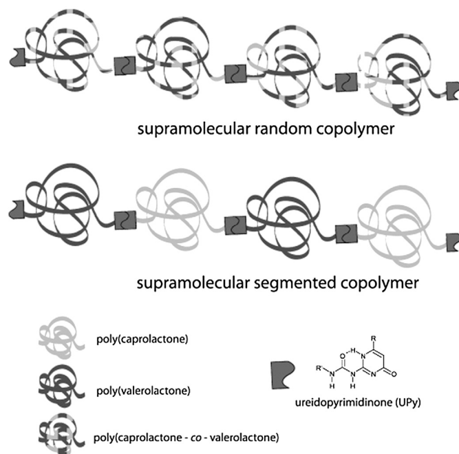
Fig. 2. Schematic drawing of supramolecular polymers formed through hydrogen bonding of ureidopyrimidinone functionalized PCL telechelics and copolymers with poly(valerolactone). Reprinted with permission from Ref. [110]. Copyright 2007 American Chemical Society.
