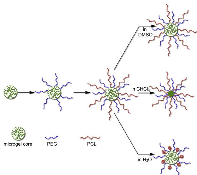
Fig. 3. Solvent dependent switching of micellar structure of a PAMAM microgel with discrete PEG and PCL chains, modified from Ref. [149]. Copyright © 2008 Wiley Periodicals, Inc.
