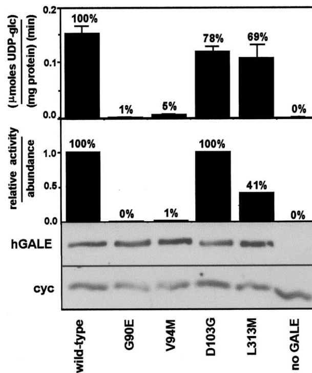
Figure 3 Activity and abundance of wild-type and mutant hGALE enzymes expressed in yeast. Top , Conversion of UDP-gal to UDP-glc detected in crude lysates of yeast expressing each of the indicated hGALE alleles in the homozygous state ( n = 3 ). Middle , Average activity values from the top panel divided by average abundance (estimated by densitometric analysis of three independent western blots), normalized to wild-type. Bottom , Representative western blot analyses of lysates probed with antisera that detect hGALE and yeast cyclophilin (an endogenous control for loading).
