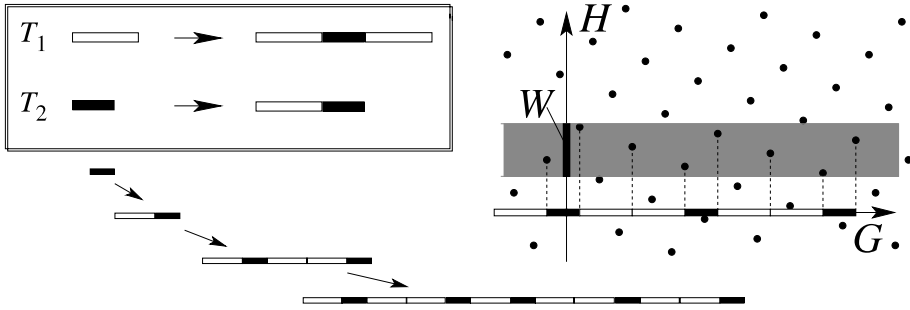
Fig. 1. The Fibonacci tile-substitution s (box top left), some iterates of s on T_2 , and the generation of a Fibonacci tiling as a cut and project tiling (right). The interval W defines a horizontal strip, all lattice points within this strip are projected down to the line.
