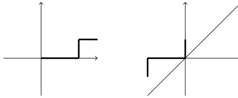
Fig. 2. The path associated with aaba (left), an example of a finite strand with coding word baab (right).
