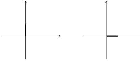
Fig. 3. The segment (0, a^*) (left) and the segment (0, b^*) (right).
