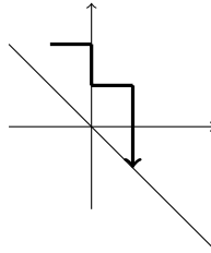
Fig. 4. An example of a finite dual strand coded by the word babaa . The arrow at the end of the path indicates that we read the letters from left to right.
