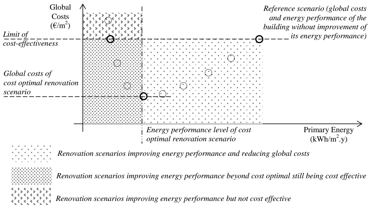
Figure 2 Cost optimal and cost effective evaluation of energy related renovation scenarios
