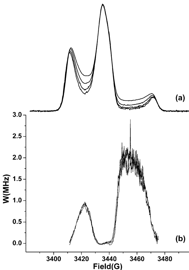
FIGURE 3 (a) Echo-detected EPR spectra of 14-PCSL in bilayer membranes of DPPC + 50 mol % cholesterol at 200 K, for interpulse spacings (top to bottom) of \tau = 216, 352, 488, and 624 \text{ ns} . Spectra are corrected for instantaneous diffusion according to Eq. 10 and are normalized to the maximum line height. (b) Anisotropic part of the relaxation rate, W , obtained according to Eq. 9 from pairs of spectra in a with interpulse separations of (top to bottom): 216 \text{ ns} and 352 \text{ ns} ; 216 \text{ ns} and 488 \text{ ns} ; and 216 \text{ ns} and 624 \text{ ns} , respectively. Note that all three curves coincide within the noise.
