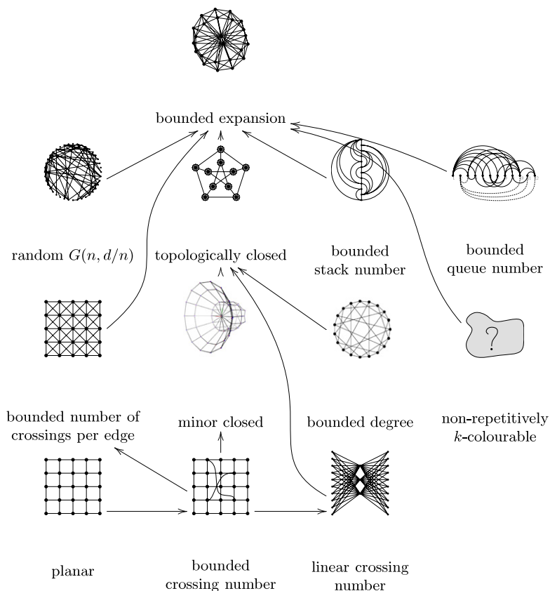
Fig. 1. Classes with bounded expansion. The results about classes with bounded crossings, bounded queue-number, bounded stack-number, and bounded non-repetitive chromatic number are proved in this paper.
