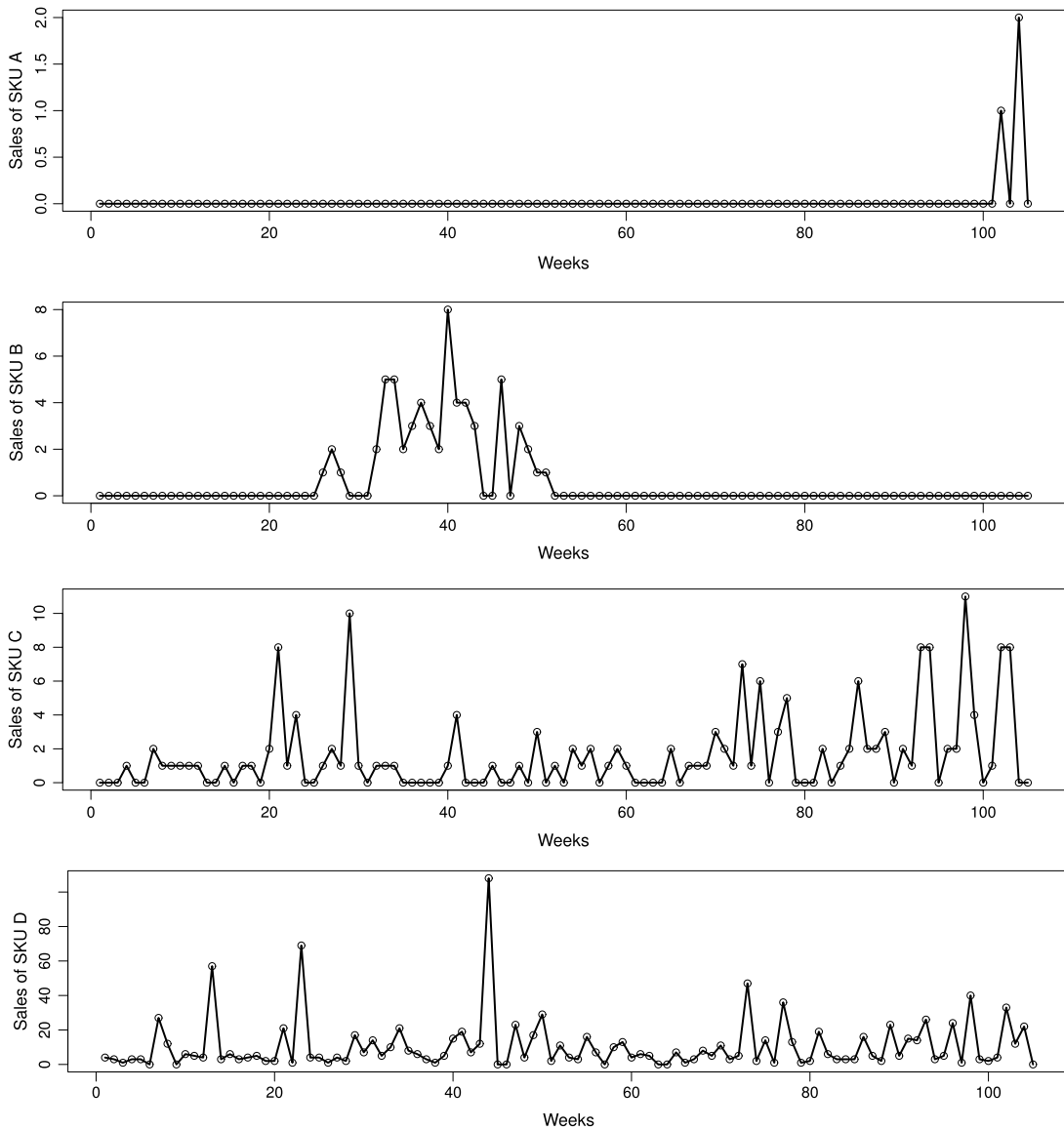
Fig. 9. Intermittent demand patterns of four SKUs in a specific store.
