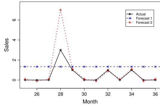
Fig. 8. Actual data and two different forecasts from the 25th to 36th months.
