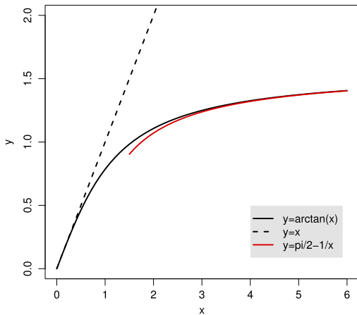
Fig. 5. For small values of x , \arctan(x) varies linearly with x , with its variation becoming nonlinear with increasing values of x ; it eventually approaches \pi/2 .
