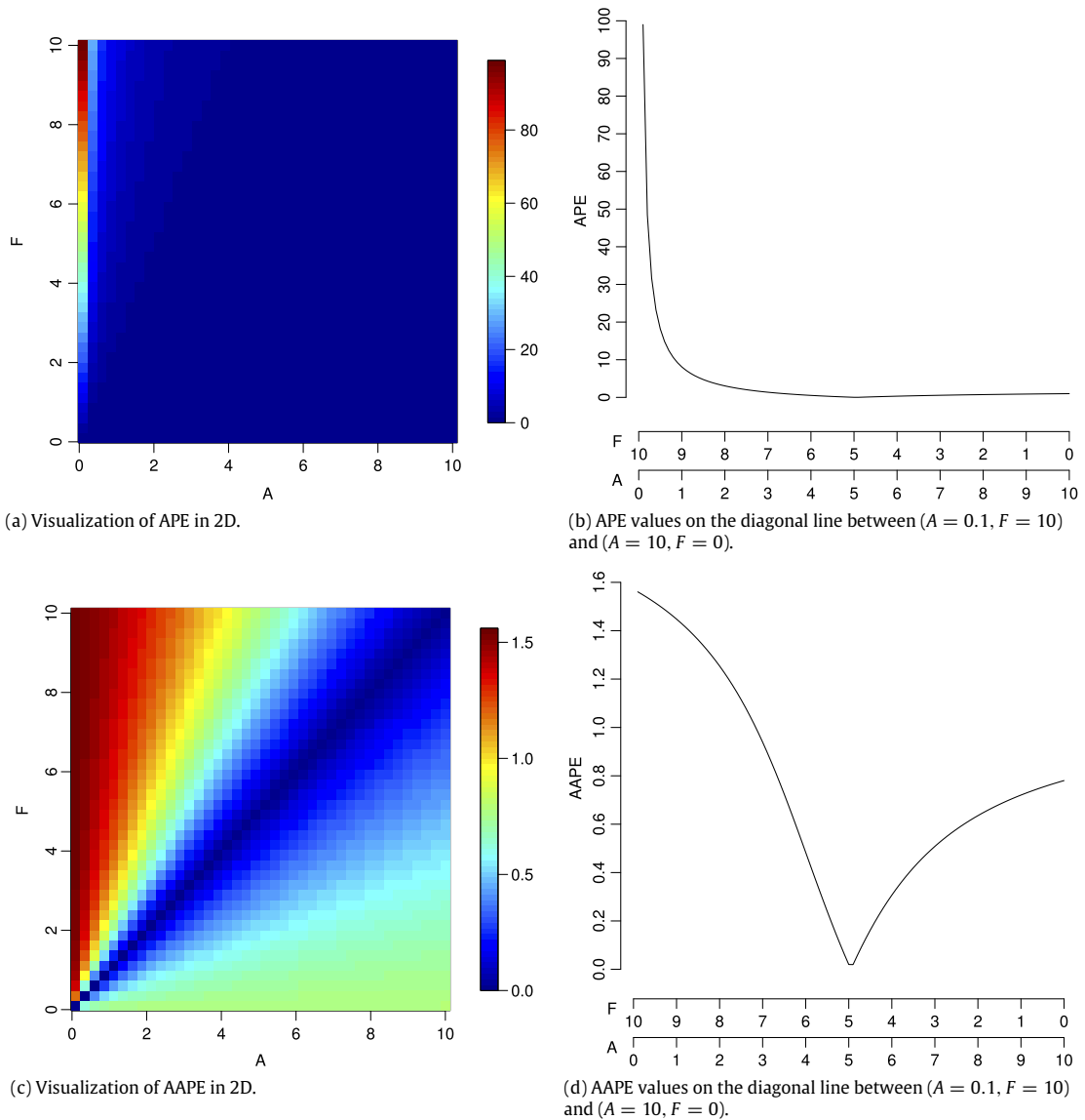
Fig. 3. Visualization of APE and AAPE on [0.1, 10] \times [0.1, 10] . (For interpretation of the references to colour in this figure legend, the reader is referred to the web version of this article.)
