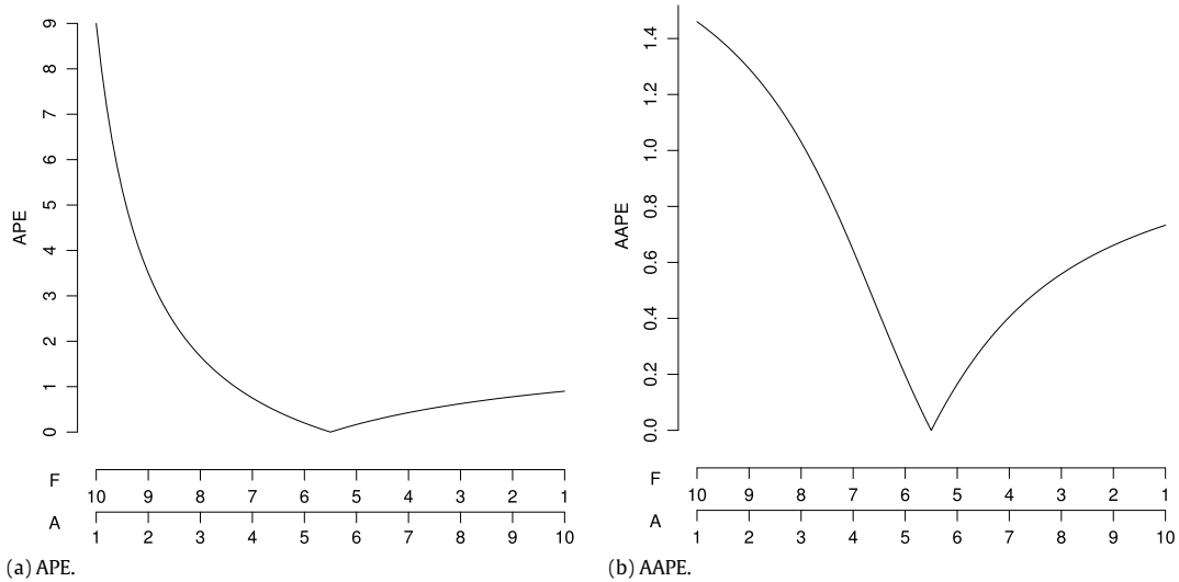
Fig. 4. Visualization of APE and AAPE on [1, 10] \times [1, 10] .
