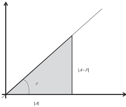
Fig. 2. Conceptual justification of AAPE: AAPE corresponds to the angle \theta , while APE corresponds to the slope as a ratio = \tan(\theta) = \left| \frac{A-F}{A} \right| , where A and F are the actual and forecast values, respectively.
