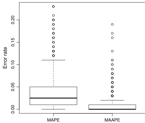
Fig. 10. Boxplots of 1000 error rates for MAPE and MAAPE.
