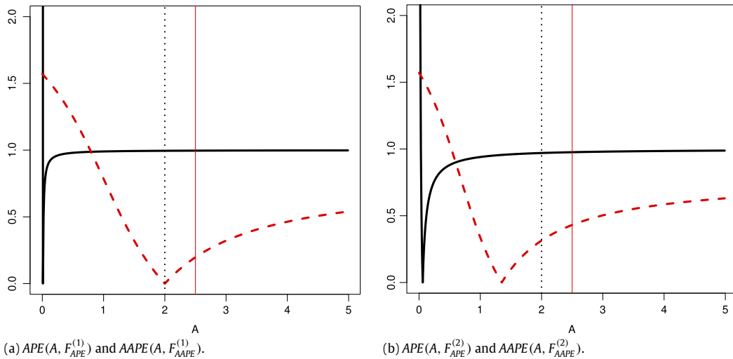
Fig. 7. Comparison between APE(A, F_{APE}^{(i)}) (black solid line) and AAPE(A, F_{AAPE}^{(i)}) (red dashed line) for (a) i = 1 and (b) i = 2 , for A that follows a negative binomial distribution ( r = 3.58, p = 0.59 ). The solid red and dotted black vertical lines indicate the locations of the mean and median of the actual demand distribution, respectively. (For interpretation of the references to colour in this figure legend, the reader is referred to the web version of this article.)
