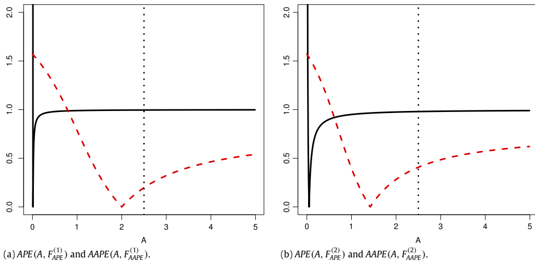
Fig. 6. Comparison between APE(A, F_{APE}^{(i)}) (black solid line) and AAPE(A, F_{AAPE}^{(i)}) (red dashed line) for (a) i = 1 and (b) i = 2 , for A that follows a discrete uniform distribution. The vertical dotted line indicates the locations of both the mean and the median of the actual demand distribution. (For interpretation of the references to colour in this figure legend, the reader is referred to the web version of this article.)
