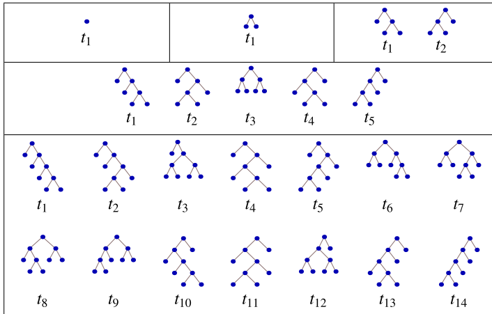
Fig. 1. The binary trees with at most 5 leaves.
