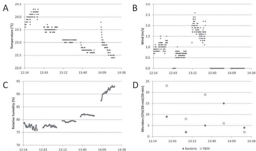
Figure 2. Atmospheric conditions in The Great Cavern of Santo Tomás from the cave entrance towards the cave interior (5, 15, 25, 100, 120 m, deep in the cave, see text for details) on 22 December 2011: A, measured air temperature; B, air inflow; C, relative humidity; D, cultivable airborne bacteria (Bacteria) and yeast and moulds (Y&M) expressed as Colony-Forming-Units CFU/20 cm 2 /20 min.
