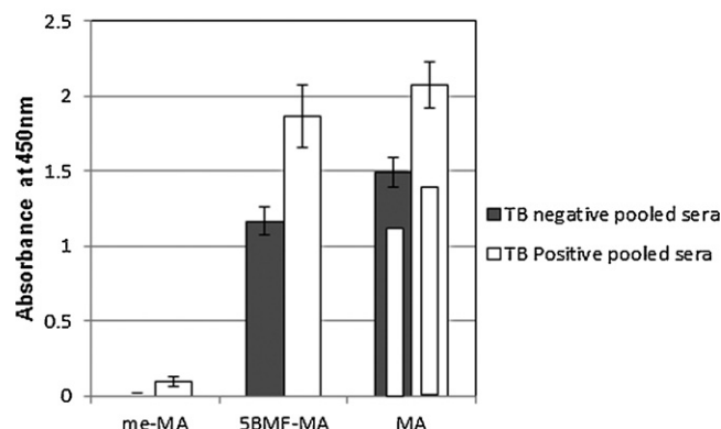
Fig. 2. Human patient antibody recognition of natural Mtb MAs (MA mix), methyl ester of natural MA (me-MA) and natural MA fluorescein ester (5BMF-MA, prepared from natural MA mix and 5BMF (structure)) measured with ELISA. Pooled TB positive and pooled TB negative sera were tested on the MA antigen derivatives coated from hexane. Inner bars within the MA mix bars indicate the signals when coating was done from hot PBS instead of hexane. The error bars indicate the standard deviation. The 2.5 d rule was applied to remove outliers. n = \text{min } 14, \text{max } 16 .
