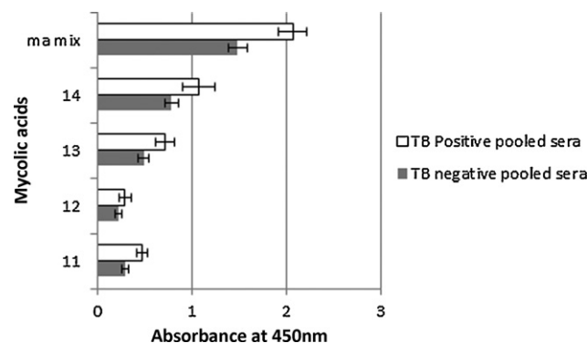
Fig. 5. ELISA antibody binding signals of pooled TB positive and TB negative sera to synthetic hydroxymycolic acids. The error bars indicate the standard deviation. The 2.5 d rule was applied to remove outliers. n = \min 15, \max 16 .
