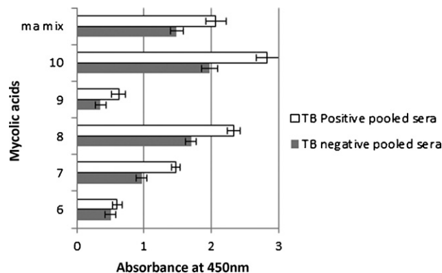
Fig. 4. Comparable ELISA signals of pooled TB positive and TB negative sera to synthetic methoxy-mycolic acids. The error bars indicate the standard deviation. The 2.5 d rule was applied to remove outliers. n = \min 14, \max 16 .
