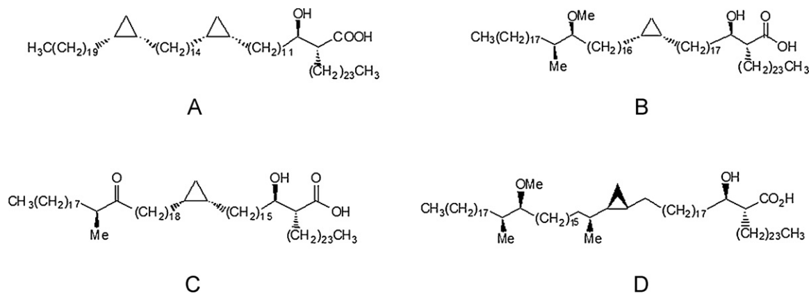
Fig. 1. Structures of the prominent homologues of three main classes of MA of Mycobacterium tuberculosis . A , alpha-; B , methoxy-; C , keto-mycolic acid; and D , the \alpha -methyl- trans -cyclopropane form of natural methoxy-mycolic acid.
