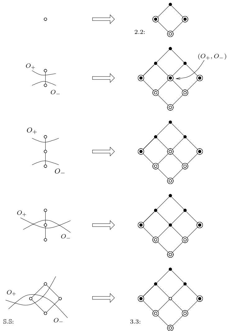
Fig. 1. Some bitopological spaces and their concrete d-frames. (D-frame elements in the con-predicate are indicated by an additional circle, those in the tot-predicate are filled in.)
