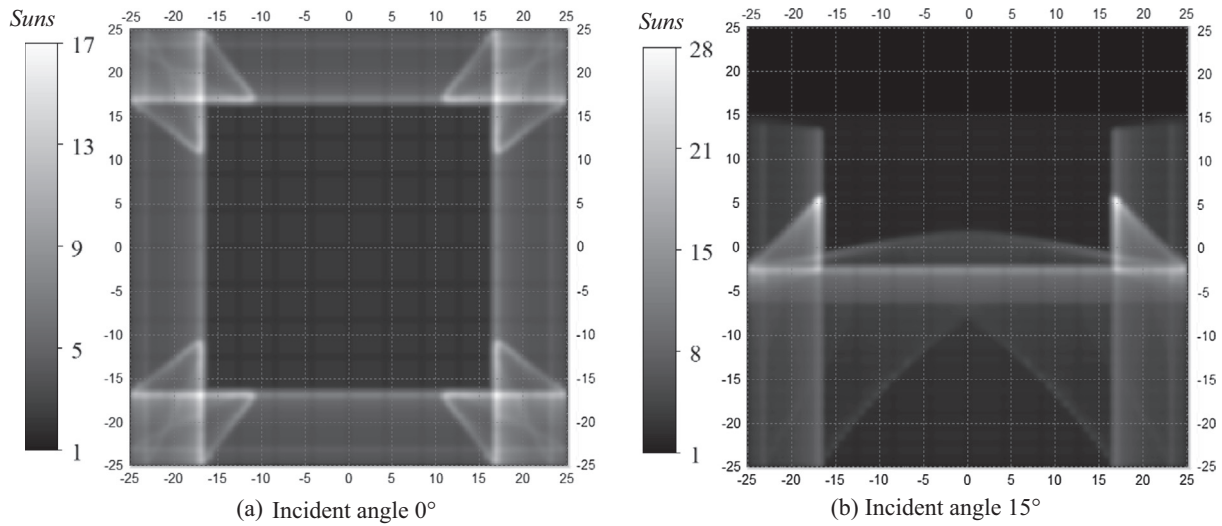
Fig. 5. The 2-D flux distributions of 3.6×/4× AR-CCPC at different incident angles, when the realistic sun model with a 4.65 mrad half angle is adopted.
