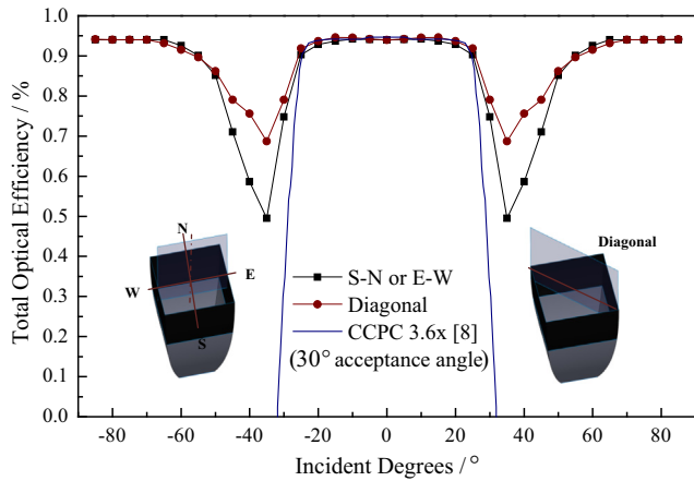
Fig. 10. A comparison of the total optical efficiency of 3.6×/4× AR-CCPC under different incident directions.
