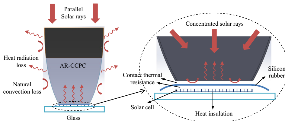
Fig. 11. The sketch of assembled AR-CCPC.
