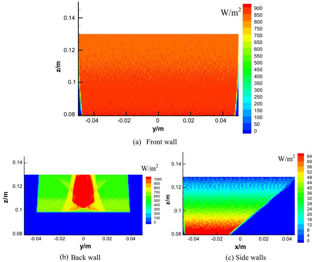
Fig. 7. The 2-D absorbed solar rays on the thermal absorber walls with an incident angle of 50^\circ , for 3.6 \times / 4 \times AR-CCPC. When the external irradiance is 1000 \text{ W/m}^2 .
