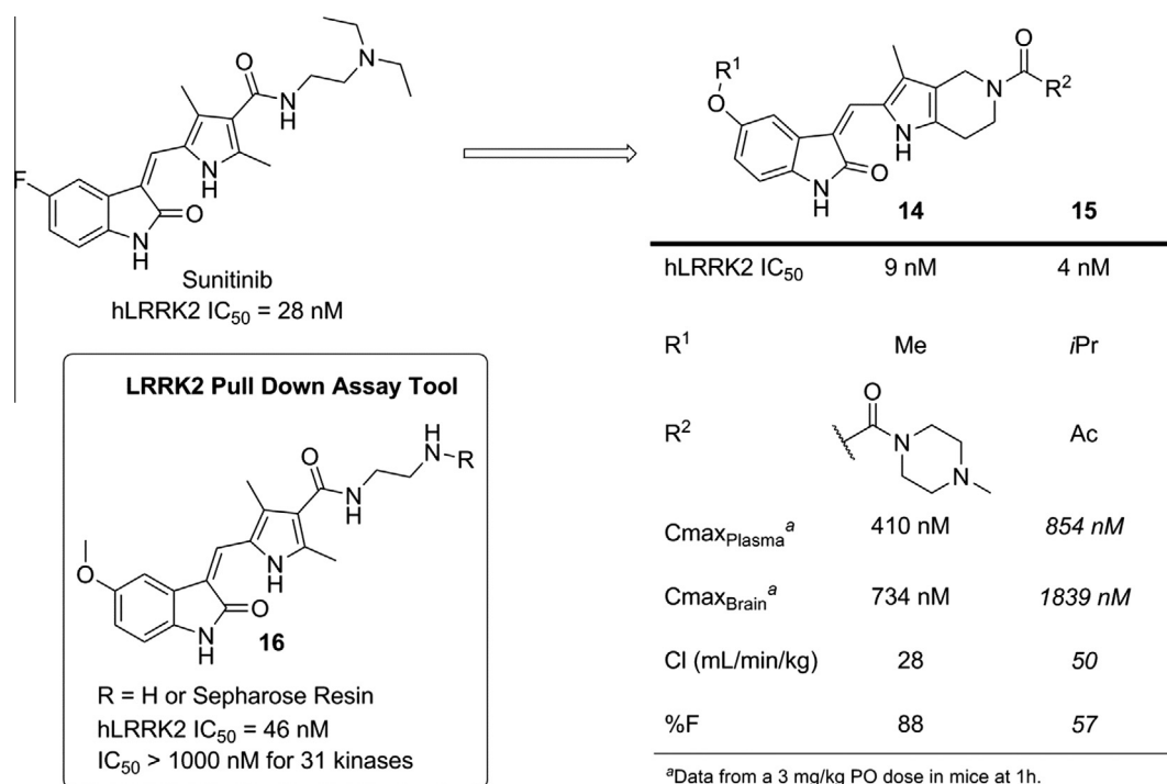
Figure 11. LRRK2 inhibitors.
