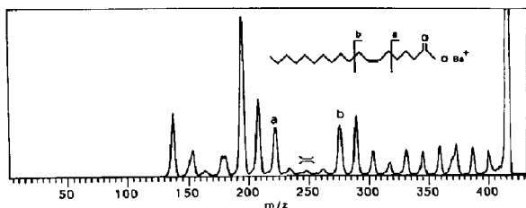
Figure 3. CAD MIKES of petroselinic acid desorbed by FAB as [M - H + Ba]^+ . The ion formed by double-bond cleavage is indicated.
