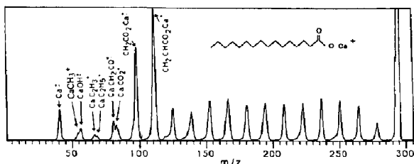
Figure 1. CAD MIKES of palmitic acid desorbed by FAB as a calcium cationized species.
