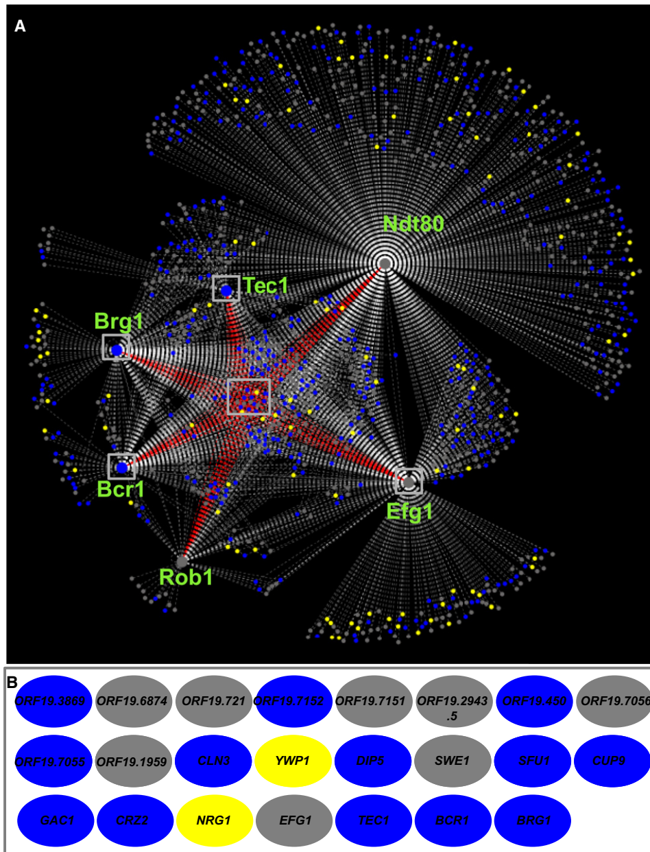
Figure 3. The Biofilm Regulatory Network
