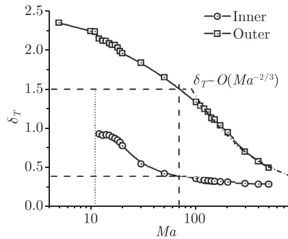
Fig. 5. Thickness of the inner and outer thermal boundary layers at different Marangoni numbers.
