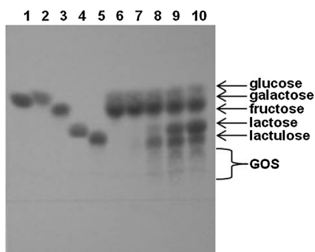
Fig. 6. TLC of products of lactulose synthesis catalyzed by Arthrobacter sp. 32cB \beta -D-galactosidase. Reaction mixtures containing lactose and D-fructose as substrates, and 2 U mL ^{-1} Arthrobacter sp. 32cB \beta -D-galactosidase were incubated at 30 ^{\circ} C for 8 h. Lane 1 – D-galactose, lane 2 – D-glucose, lane 3 – D-fructose, lane 4 – lactose, lane 5 – lactulose, lane 6 – reaction mixture containing 29 mM of each substrate, lane 7 – reaction mixture containing 58 mM of each substrate, lane 8 – reaction mixture containing 146 mM of each substrate, lane 9 – reaction mixture containing 292 mM of each substrate, and lane 10 – reaction mixture containing 438 mM of each substrate.
