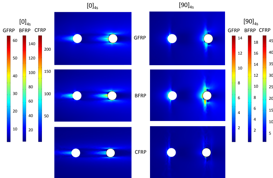
Fig. 11. Comparative analysis. Equivalent von Mises stress (in MPa) distribution at the failure state close to the pin-plate interfaces, for the 1-2-B joint configuration.
