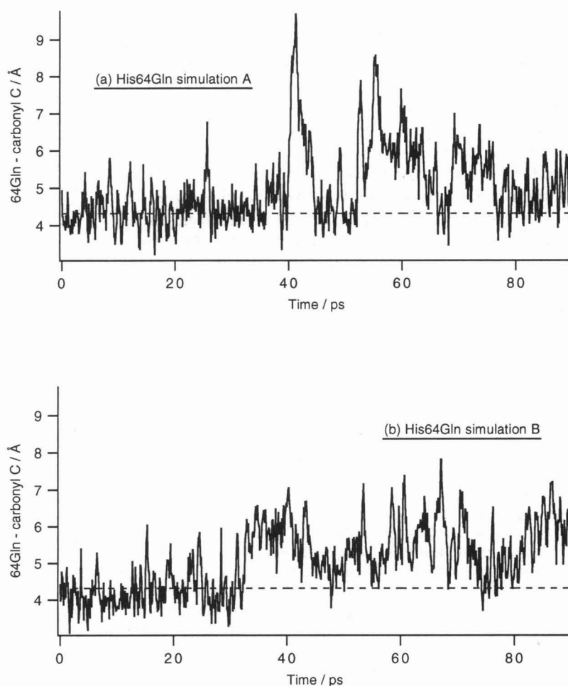
FIGURE 2 Separation between the 64Gln side chain (defined as the average of the C_\gamma , C_\delta , N_\epsilon , and O_\epsilon positions at a given time t ) and the carbonyl C for the His64Gln trajectories. The dotted line shows the separation, 4.32 Å, in the x-ray structure (PDB file 2MGF).
