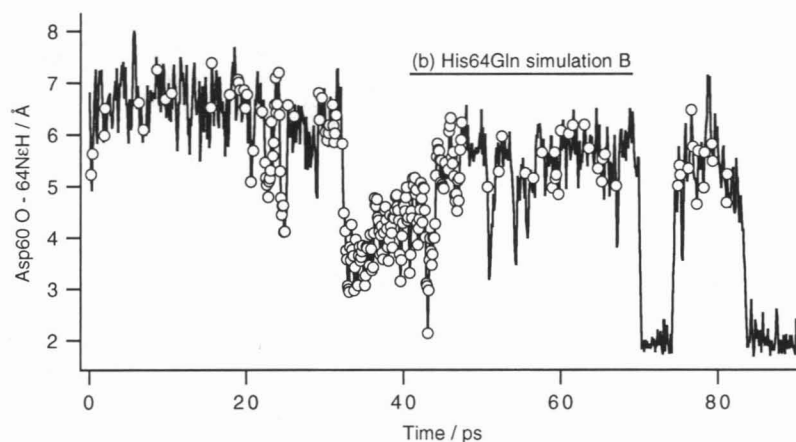
FIGURE 6 Separation between the distal N_\epsilon H hydrogens and the Asp60 main chain O during the two His64Gln trajectories; only the nearest of the two hydrogens is shown for any given time t (open circles correspond to the hydrogen cis to the 64O_\epsilon oxygen; otherwise the trans hydrogen is closest). The separation found in the “open” conformation of the wild type 64N_\delta H tautomer is shown for comparison (Jewsbury and Kitagawa, 1994).
