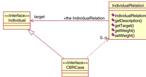
Fig. 2. Case representation.
