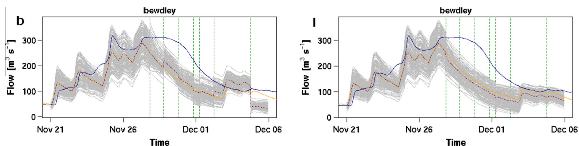
Fig. 5. Inflow estimation at Bewdley for filters with configuration (b) and (l), as specified in Table 2.
