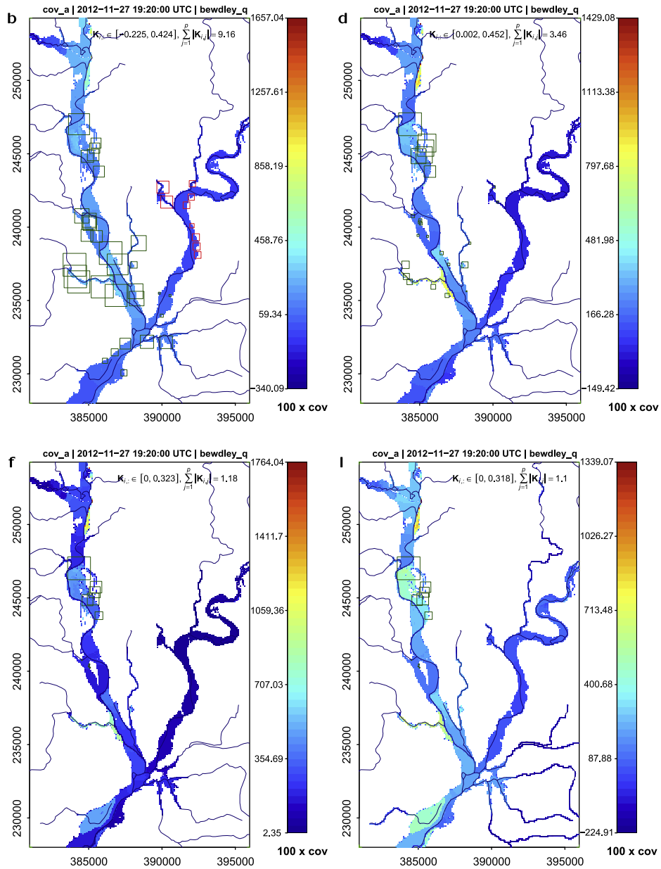
Fig. 6. Updated error covariance between the inflow boundary conditions at Bewdley and the state vector (water level elsewhere) at the first assimilation step (1th CSK overpass) for the same filter than Fig. 4. Plots focus on the satellite coverage area, thus Bewdley location is not shown. Description is as Fig. 4, being now i the state vector index corresponding to inflow errors at Bewdley.
