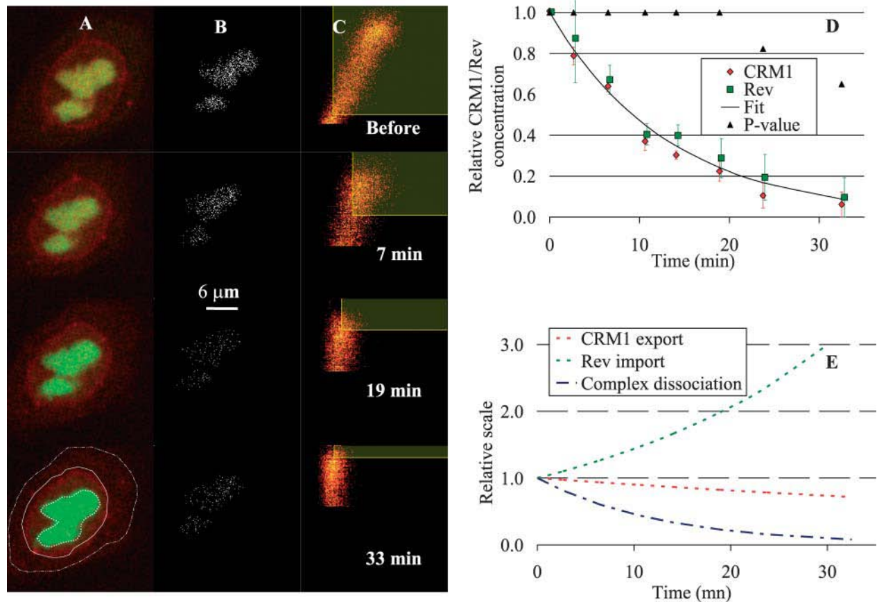
FIGURE 5 Rev-CRM1 dissociation. (A) Time series of two-dimensional confocal sections of a cell cotransfected with CRM1 and Rev fused to YFP (red) and CFP (green), respectively. (B) The corresponding estimate of colocalized pixels (shown in white). (C) The corresponding two-dimensional histograms for each image in A. The red channel (CRM1) is on the x axis and the green one (Rev) on the y axis in the two-dimensional histogram. Selected colocalized areas are also shown by yellow transparent rectangular areas. Initially, CRM1 colocalized with Rev in the nucleolus. Thirty-three minutes after addition of leptomycin B, an inhibitor of the CRM1-cargo binding, most of the CRM1 has dispersed in the nucleus. The last image of the color sequence indicates the region of the nucleolus in which the amount of colocalization is computed (bold dashed line in A). The nucleus and cell limits are also shown (solid and light dashed lines, respectively, in A). (D) The graph shows the relative concentration of the bound complex Rev/CRM1 derived from the amount of colocalization of each protein (expressions in Eq. 12) as a function of time after the end of the lag period. The dissociation rate constant k_d was found to be (1.25 \pm 0.31) \times 10^{-3} \text{ s}^{-1} (fit shown by solid line). Error bars are standard errors based on all cells averaged for each time point. Average P -values for colocalization significance test are also plotted as \blacktriangle and confirm Rev/CRM1 interaction for at least the first 20 min of dissociation (at a 95% significance level). These results match very well the two-dimensional histogram shown in C, where the linear behavior goes from a clear inclined line to a vertical line at 33 min, indicating no more colocalization. (E) shows the least-square fits of the import rate of Rev into the nucleolus and the diffusion of CRM1 out of the nucleolus after injection of LMB versus the dissociation rate obtained in D, which clearly indicates that simply measuring the loss of CRM1 outside the nucleolus after injection of LMB had nothing to do with measuring the dissociation of Rev/CRM1.
