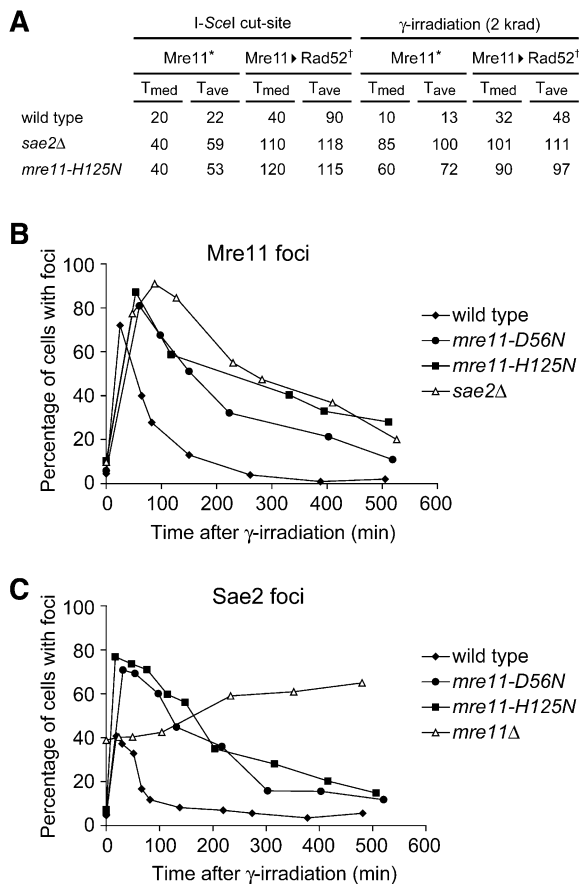
Figure 5. Kinetics of Mre11, Rad52, and Sae2 Foci (A) Summary of time-lapse microscopy of Mre11 and Rad52 foci after I-SceI cleavage or \gamma -irradiation. *, median (T med ) and average (T ave ) duration of Mre11 foci. †, time from Mre11 appearance to Rad52 recruitment. See Supplemental Figure S3 (available on Cell website) for details. (B) Kinetics of Mre11 focus formation after 40 Gy of \gamma -irradiation. Strains W3483-10A ( MRE11-YFP ), W3750-1B ( MRE11-YFP sae2 \Delta ), W5549-4A ( mre11-D56N-YFP ), and W5536-3A ( mre11-H125N-YFP ) were used in the experiment (C) Kinetics of Sae2 focus formation after 40 Gy of \gamma -irradiation. Strains W4249-5C ( SAE2-YFP ), W4249-6B ( SAE2-YFP mre11 \Delta ), W5579-15B ( SAE2-YFP mre11-D56N ), and W5578-2B ( SAE2-YFP mre11-H125N ) were used in the experiment.
