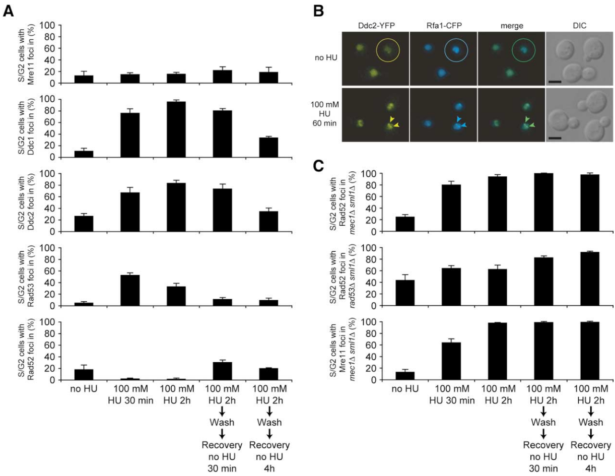
Figure 6. Induction of Checkpoint and Repair Foci by Stalled or Collapsed Replication Forks
