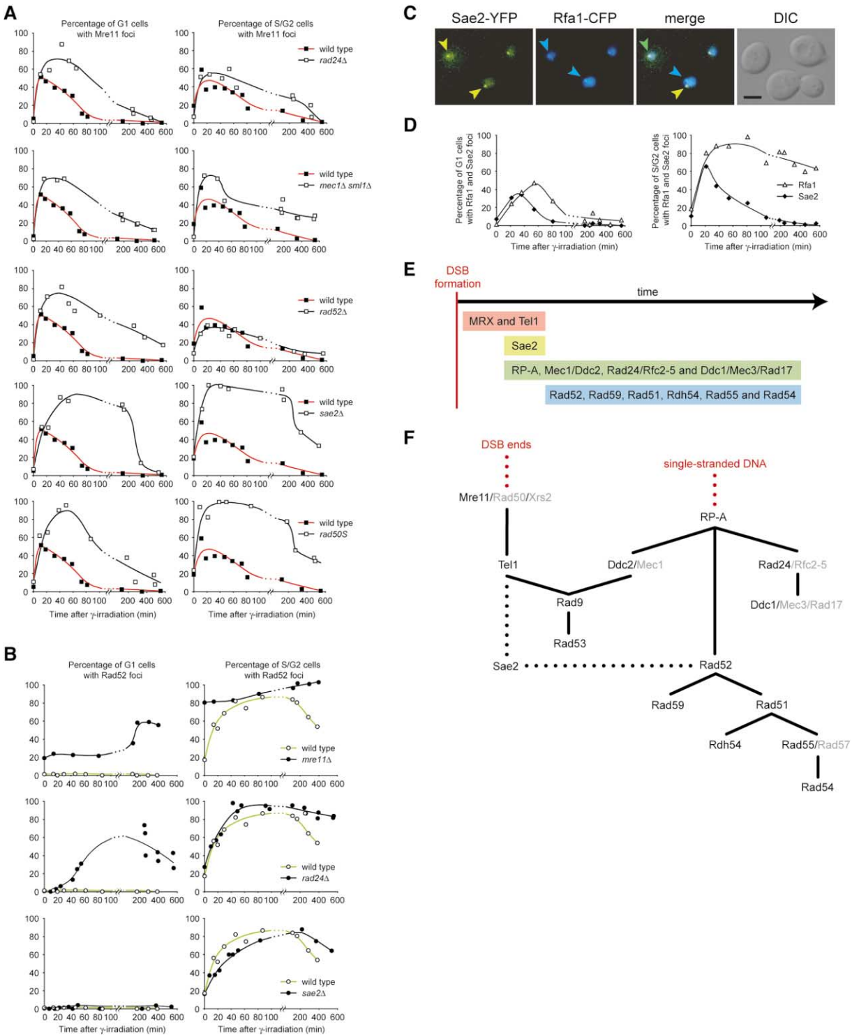
Figure 4. Choreography of Checkpoint Activation and DNA Repair
