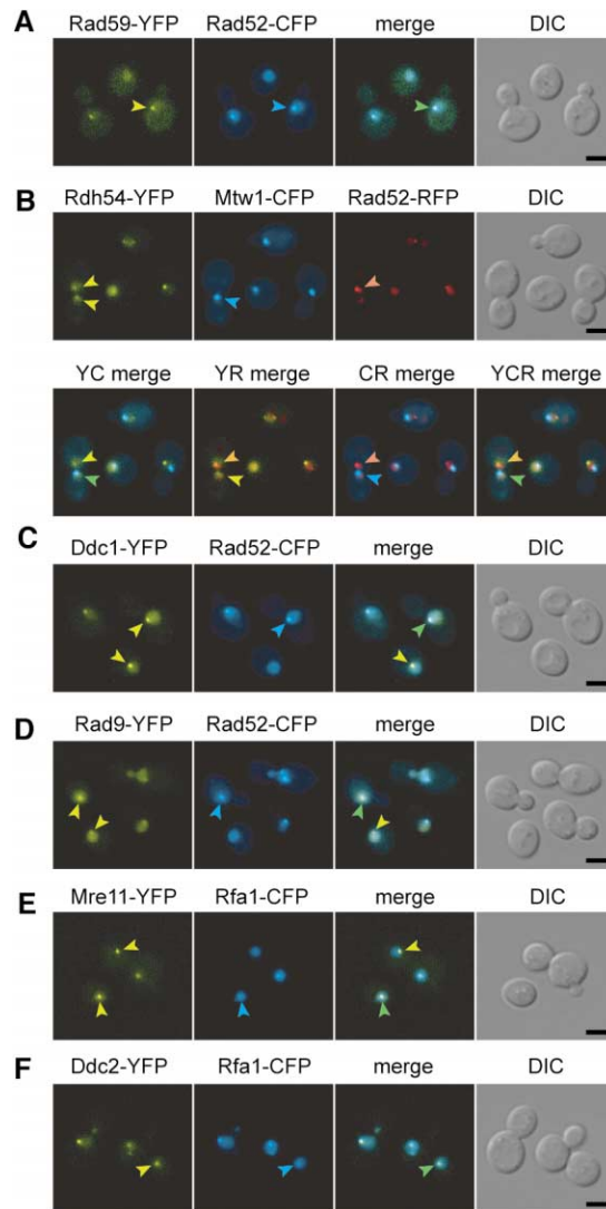
Figure 1. Colocalization of Checkpoint and Repair Foci
