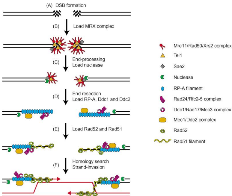
Figure 7. Model for Recruitment of Checkpoint and Recombination Proteins to a DSB (A–B) DSB formation and recruitment of the MRX complex, Tel1, and Sae2. (C) The MRX complex initially processes the DSB ends and dissociates as 5′-3′ resection is initiated by an unknown nuclease(s). (D) Single-stranded DNA generated by resection is bound by RP-A, which recruits the Ddc2/Mec1, Rad24/Rfc2-5, and Ddc1/Rad17/Mec3 complexes. (E–F) Only after cells have entered S phase is Rad52 recruited to DSB ends to catalyze the displacement of RP-A by Rad51, which is a prerequisite for strand invasion.
