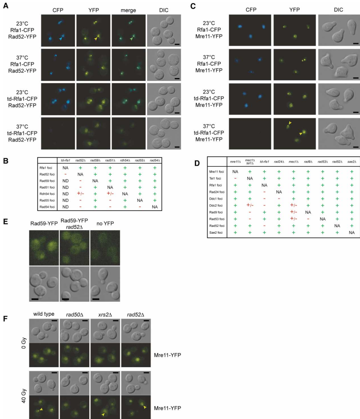
Figure 2. Genetic Requirements for Focus Formation
