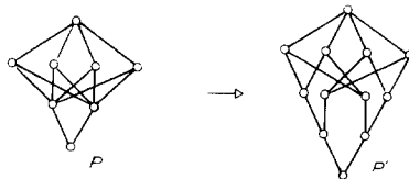
FIG. 4.1. Construction of a poset demonstrating \mu_{\text{ub}}(2, 3) \geq 3 .
