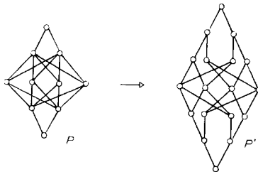
FIG. 4.2. Construction of a poset demonstrating \mu_{\text{bd}}(2, 5) \geq 3 .
