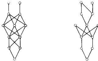
FIG. 3.1. Two ranked posets \hat{P} with maximal |\mu(\hat{P} \oplus \hat{1})| = 2 (and t' = 4 respectively t' = 3 ) for given rank generating function 1 + 2p + 2p^2 + 3p^3 + 2p^4 + 2p^5 .
