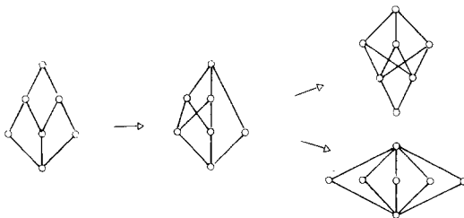
FIG. 2.1. Two alternative sequences of posets P \rightarrow P' \rightarrow P'' as generated in the proof of Theorem 2.5, with \mu(P) = \mu(P') = 0 and \mu(P'') = -2 (top) (resp. \mu(P'') = 4 (bottom)).
