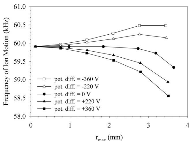
Figure 10. Frequency of ion motion along the x = 0 vector of the electrode array shown in Figure 1. The frequency of motion was obtained by fast Fourier transforming the 25 ms ion trajectory used in the simulation. The data were plotted against the dc potential difference applied to the auxiliary electrodes and the maximum radial amplitude that the ion sampled during the trajectory.
