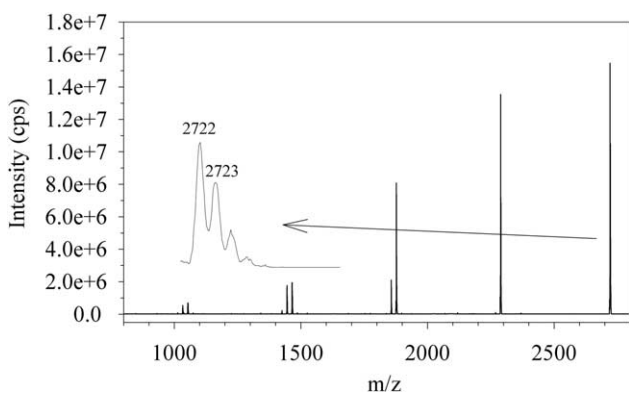
Figure 2. Fragmentation pattern observed for excitation of m/z = 2722 Th at 59.580 kHz. The excitation period was 100 ms, excitation amplitude was 255 mV o-p and the excitation q was \sim 0.205 . The auxiliary electrodes were held at +220 V relative to the quadrupole dc potential offset.
