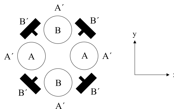
Figure 1. The electrode geometry used to create the dc octopole field. The A and B poles are the normal quadrupole rods. The letters A' and B' represent the positions of the A and B poles for the octopole. Applying a dc potential to the "T"-shaped electrodes creates the dc octopolar field.
