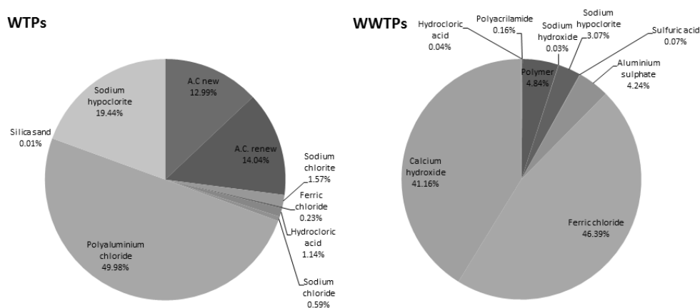
Fig. 4. Annual GHG emissions from production of chemicals consumed in Turin Metropolitan Area UWC, year 2012.
