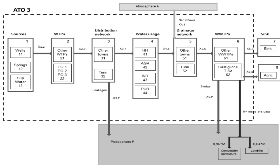
Fig. 2. ATO3 Urban Water Cycle.
