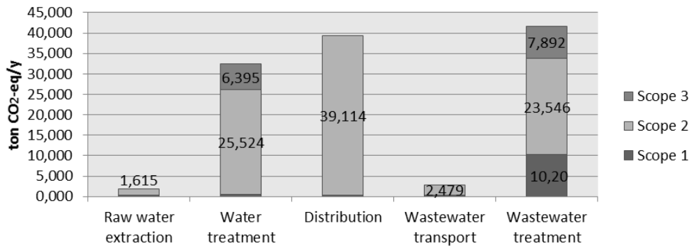
Fig. 5. Total annual GHG emissions of Turin Metropolitan Area UWC (year 2012).
