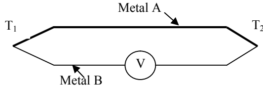
Fig.2 Thermoelectric generation based on Seebeck effect
