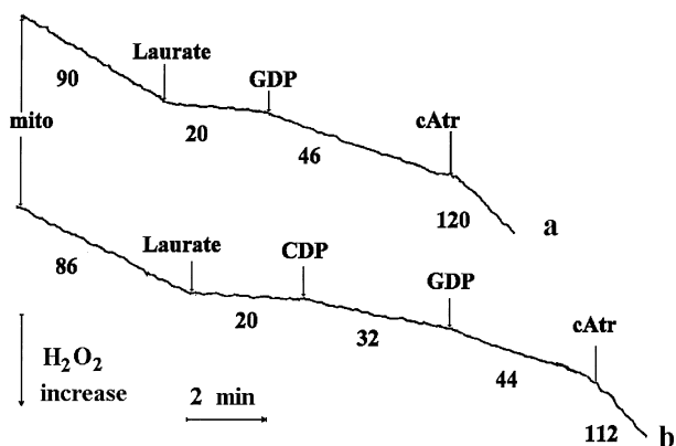
Fig. 2. Effect of cAtr and GDP on H_2O_2 generation by heart muscle mitochondria from rats exposed for 2 days to 6°C. For conditions, see Fig. 1. GDP and CDP concentrations were 0.5 mM.
