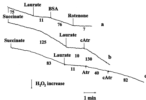
Fig. 1. Effect of laurate on H_2O_2 generation by rat heart mitochondria. The incubation medium contained 0.25 M sucrose, 10 mM MOPS (pH 7.3), 0.5 mM EGTA, 10 mM KCl, horseradish peroxidase (25 U), 1.2 \times 10^{-6} M scopoletin, 5 mM succinate and rat heart mitochondria (1 mg protein/ml). Additions: 5 \times 10^{-6} M laurate; BSA, 0.5 mg/ml; 2 \times 10^{-7} M rotenone; 2 \times 10^{-6} M cAtr; 6 \times 10^{-6} M Atr. Figures near curves are rates of H_2O_2 production (pmol of H_2O_2 /mg protein/min).
