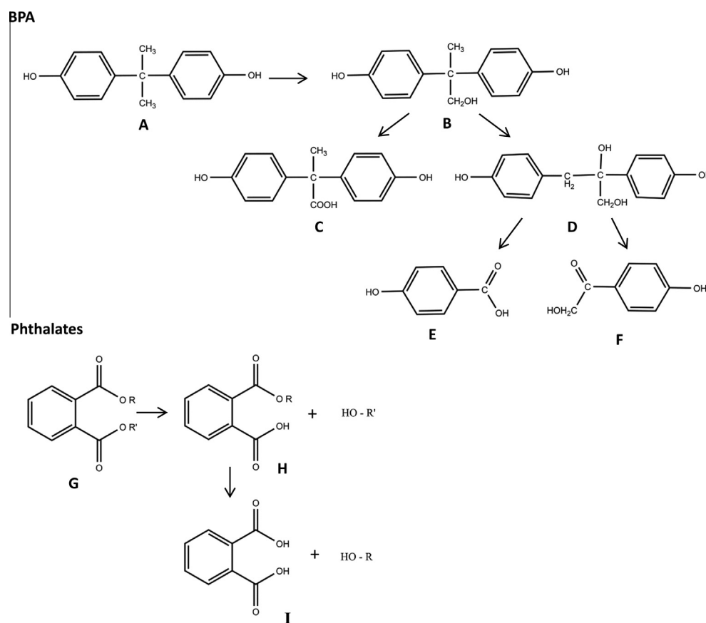
Fig. 1. Examples of biological degradation pathways of BPA and phthalates. (A) BPA consists of two aromatic rings with a hydroxyl group on either end. (B) One methyl group of BPA is oxidized to form 2,2-bis(4-hydroxyphenyl)-1-propanol (C) and further transforms to intermediate metabolites 2,2-bis(4-hydroxyphenyl)propanoic acid (D) and tetraol. (E) Tetraol is further degraded to 4-hydroxybenzoic acid (F) and 2-hydroxy-1-(4-hydroxyphenyl) ethanone. Adapted from Suzuki et al. (2004a). (G) Ortho -phthalate diesters have an aromatic ring and two esters on adjacent carbons. (H) Diesters are metabolised into phthalate monoesters and alcohol. (I) Further degradation yields phthalic acid and alcohol. The resulting alcohols are of added concern due to their high volatility. For most ortho -phthalates, the degradation is incomplete and results in a mixture of monoesters, alcohols and phthalic acid. Adapted from Horn et al. (2004) and Liang et al. (2008).
