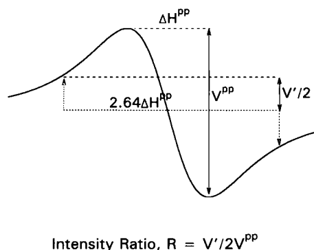
FIGURE 1 Definition of the peak-to-peak linewidth, \Delta H^{PP} , and of the intensity ratio, R , of a first-derivative display of an electron spin resonance spectral line. See text and Sankaram et al. (1992), Bales (1980, 1982, 1989) for further details of the intensity ratio.
