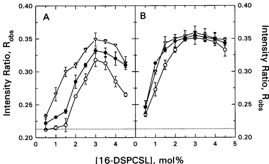
FIGURE 5 Dependence on the concentration of 16-DSPCSL of the intensity ratio, R_{obs} , of the middle hyperfine line in the ESR spectrum of 16-DSPCSL. Data were obtained from (A) 50:50 (mol/mol) mixtures of DMPC/DSPC and (B) 40:60 (mol/mol) mixtures of DMPC/DSPC. In A the temperatures are 32°C (○), 34°C (●), and 38°C (▽), and in B, they are 34°C (○), 38°C (●), and 42°C (▽). The dashed line in both A and B is the maximum value for the intensity ratio, R^L = 0.213 , for a Lorentzian line (Sankaram et al., 1992).
