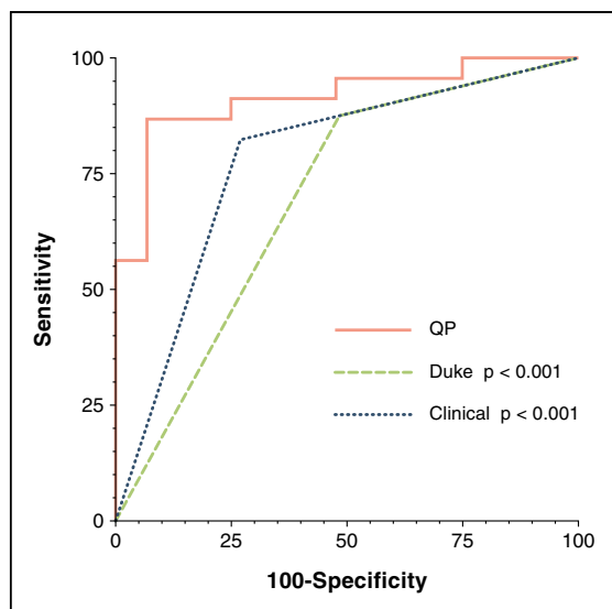
Figure 3. ROC Curves of QP and Qualitative Methods
