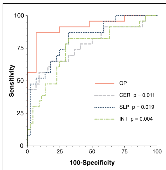
Figure 1. ROC Curves of QP and Semiquantitative Methods
