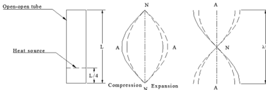
Fig. 2. Pressure oscillation and velocity (change of displacement) oscillations in Rijke tube [7].
