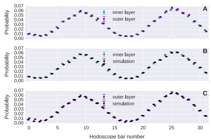
Fig. 6. Angular distribution of cosmic rays as recorded with the hodoscope detector. The bar numbers 0 to 31 cover 360°. A: Comparison of data for the inner and the outer hodoscope. p=0.998 . B: Comparison of inner hodoscope data with simulations. p=0.999 . C: Comparison of outer hodoscope data with simulations. The data are normalised as probabilities. p=0.992 .
