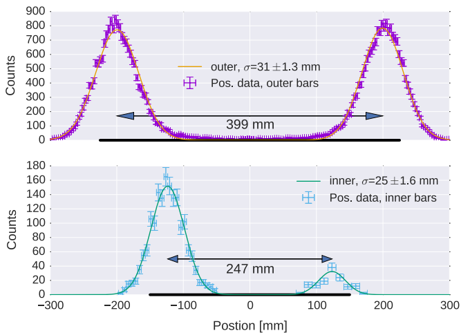
Fig. 4. Measurements for determining the position resolution for both hodoscope bars. The two peaks correspond to the positions of a reference scintillator, indicated by the arrow. The length of the hodoscope bar is represented by the black line on the abscissa. Top: position resolution for the outer hodoscope bars with Gaussian ODR. Bottom: position resolution for the inner hodoscope bars with Gaussian ODR. The asymmetry between the two peaks for the inner hodoscope arises from the reduced measurement time for the second peak.
