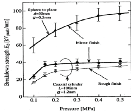
Fig. 3 Pressure dependence of breakdown strength in LN 2 gap
