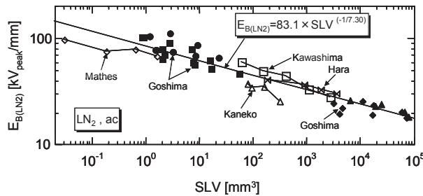
Fig. 2 Volume effect of breakdown strength in LN 2 gap
