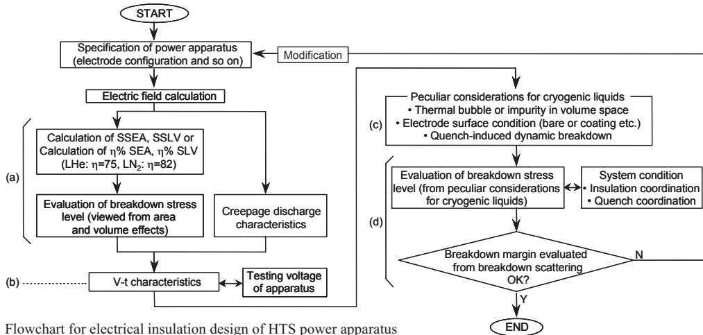
Fig. 1 Flowchart for electrical insulation design of HTS power apparatus (“SSEA” and “SSLV” are statistical stressed electrode area and liquid volume. “ \eta % SEA” and “ \eta % SLV” are stressed electrode area and liquid volume against the maximum electric field strength. “V-t (characteristics)” is “Voltage - time (characteristics)”.)
