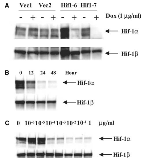
Fig. 3. Tetracycline dependent target knockdown in stable cell lines using the 2O2 expression system. (A) HeLa-TREx stable cell lines with integrated 2O2 vector (vec1, vec2) or 2O2_Hif1(Hif1-6, Hif1-7) were treated with 1 \mu g/ml doxycycline for 24 h followed by 6 hour treatment with 100 \mu M DFO. (B) Hif1-7 cells were treated with 1 \mu g/ml of doxycycline for indicated time before being treated with 100 \mu M DFO for 6 h. (C) Hif1-7 cells were treated with different concentrations of doxycycline for 48 h followed by 6 h treatment with 100 \mu M DFO. After treatment, cells were lysed and analyzed by Western blotting using an antibody against Hif1 \alpha or Hif1 \beta .
