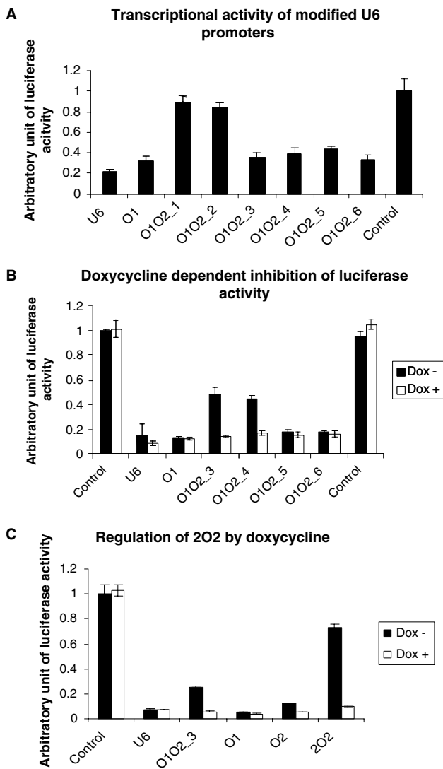
Fig. 2. Transcriptional activity and tetracycline response of U6 promoter variants. (A) The plasmids that use each U6 promoter variants to express shRNAs are designated as U6_luc, O1_luc, O1O2_luc1, O1O2_luc2, O1O2_luc3, O1O2_luc4, O1O2_luc5, and O1O2_luc6. 0.008 \mu g each of these plasmids or a control vector was cotransfected with 1 \mu g pGL3-control and 0.5 \mu g pRL-TK. Luciferase activities in transfected cells were determined 72 h post transfection. (B) 0.2 \mu g each of a control plasmid, U6_luc, O1_luc, and O1O2_3–6 was cotransfected with 1 \mu g pGL3-control, 0.5 \mu g pRL-TK and 1 \mu g of pcDNA6/TR. (C) 0.2 \mu g each of a control plasmid, U6_luc, O1O2_3, O1_luc, O2_luc, or 2O2_luc was cotransfected with 1 \mu g pGL3-control, 0.5 \mu g pRL-TK and 1 \mu g of pcDNA6/TR. For doxycycline treatment, cells were changed to culture medium containing 1 \mu g/ml of doxycycline 24 h post transfection. Luciferase activities were determined 48 h after induction by doxycycline.
