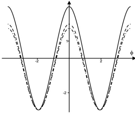
Fig. 1. Plots of the potential (53) for b = \sqrt{6}/3 , a = 1 and for \alpha = 0.1 (solid line), \alpha = 1 (dashed line) and \alpha = 10 (dot-dashed line).
