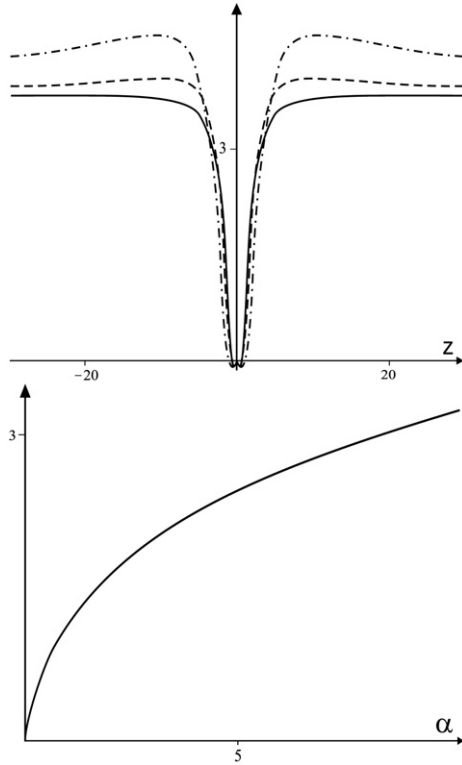
Fig. 4. Plots of z^2U(z) for the type I model (upper panel) for \alpha = 0.1 (solid line), \alpha = 1 (dashed line) and \alpha = 10 (dot-dashed line), showing the asymptotic regime for large z . We use b^2 = 2/3 . We also plot the ratio M_4^2/M_*^3 (lower panel) between 4-dimensional coupling and fundamental 5-dimensional Planck scale as a function of \alpha .
